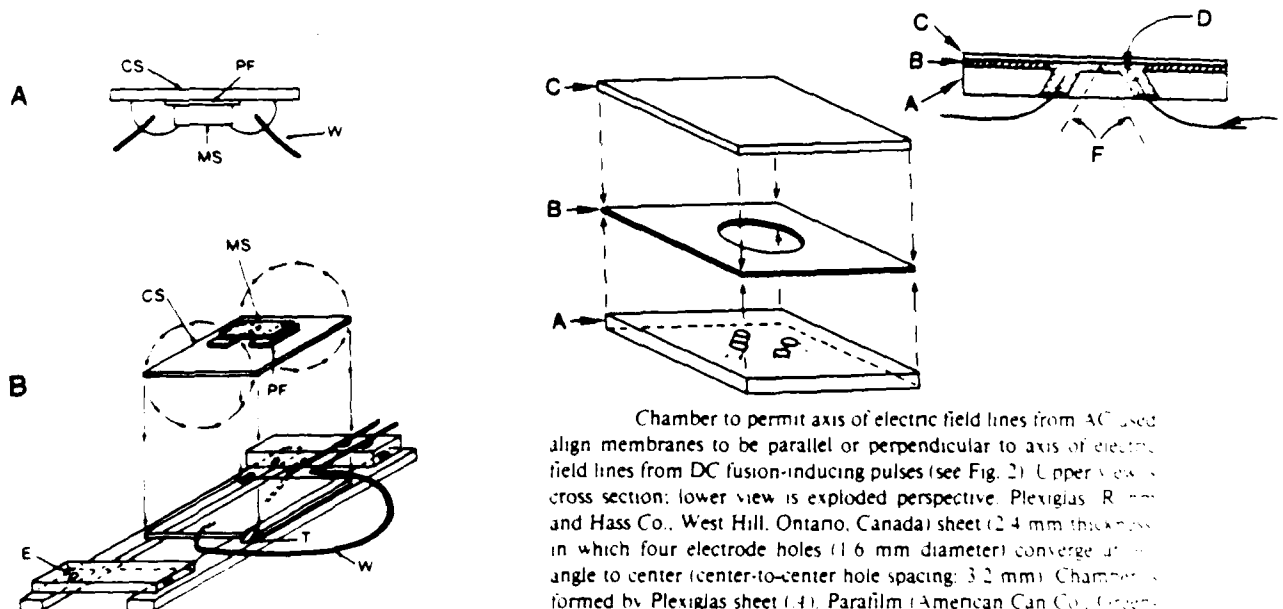
FIGURE 1. Fusion chamber. (A) Fusion chamber made by heat sealing of a microslide (MS) with parafilm (PF) in a dry mounting press to a coverslip (CS). (B) Fusion chamber mounted with tape (T) in a frame made from glass strips cut from a standard microscope slide and cemented together with epoxy cement (E). Wire electrodes (W) are anchored to the frame with epoxy cement.
