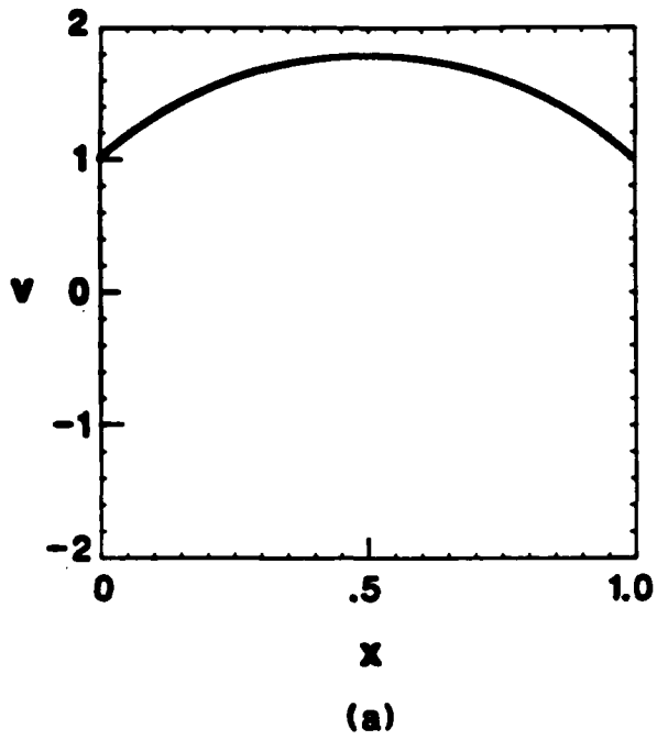
Fig. 5. Phase space at end of run and history of E_0 for short circuit case with \alpha = 3\pi/2 . (Phase space plot is actually comprised of many particles, and not a single curve, as it appears.)
