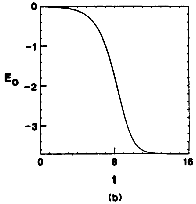
Fig. 5. Phase space at end of run and history of E_0 for short circuit case with \alpha = 3\pi/2 . (Phase space plot is actually comprised of many particles, and not a single curve, as it appears.)
