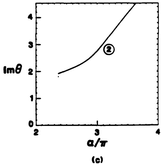
Fig. 19. Dispersion curves for dominant modes of non-uniform equilibrium for C = 20 . Mode which is dominant for 2 < a/\pi < 3 is purely growing.
