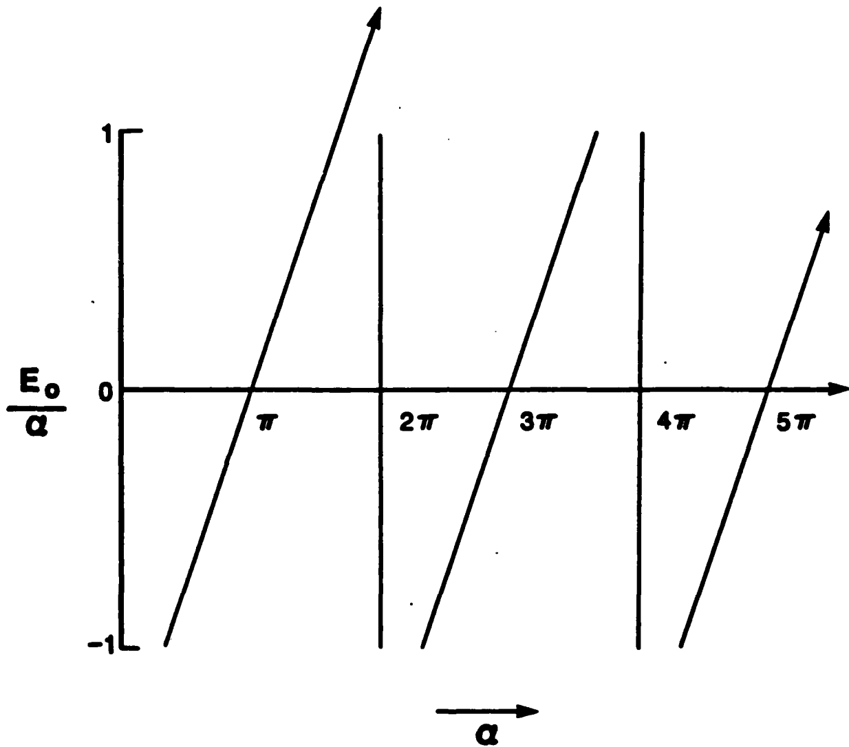
Fig. 2. Non-uniform equilibria for short circuit ( C = \infty ) case. All lines end at |E_0| = \alpha , except for first line (with arrow), which extends indefinitely.
