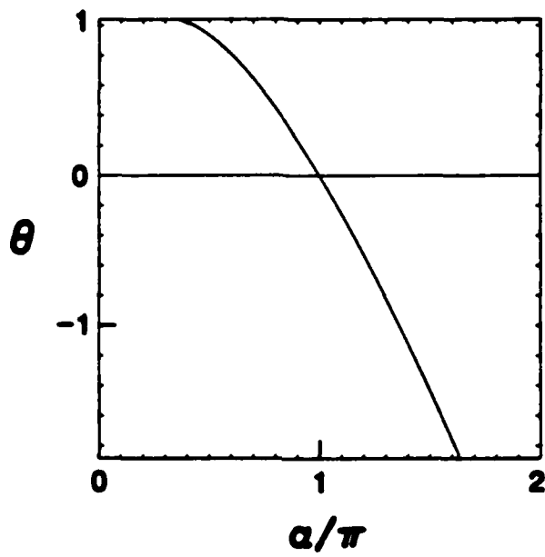
Fig. 15. Dispersion curve for dominant mode of non-uniform equilibrium in short circuit case for 0 < \alpha < 2\pi ( Im \theta is zero for this mode)
