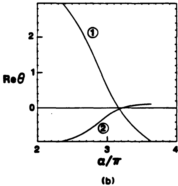
Fig. 19. Dispersion curves for dominant modes of non-uniform equilibrium for C = 20 . Mode which is dominant for 2 < a/\pi < 3 is purely growing.
