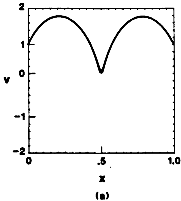
Fig. 6. Phase space at end of run and history of E_0 for short circuit case with \alpha = 7\pi/2
