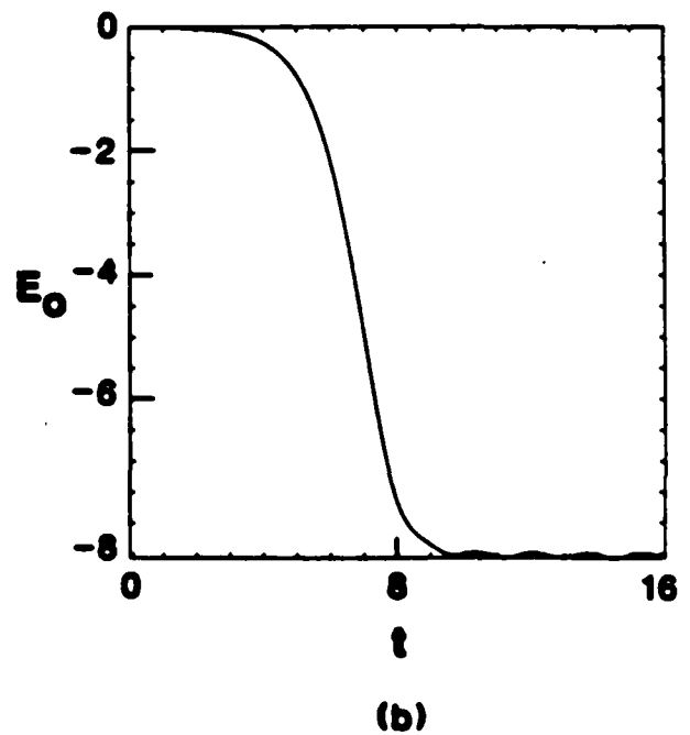
Fig. 6. Phase space at end of run and history of E_0 for short circuit case with \alpha = 7\pi/2
