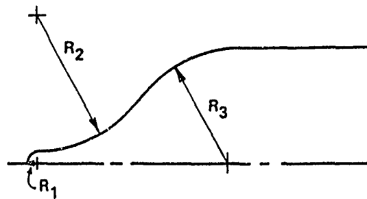
Figure 4b TRI-RADIUS REPRESENTATION FOR ABLATED NOSE SHAPE
