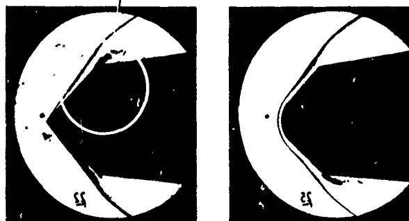
Figure 47 Schlieren Photographs of the Flow Over the Sharp Biconic Nosetip Showing the Individual Shocks for the Roughness Elements (Ref. 61)
