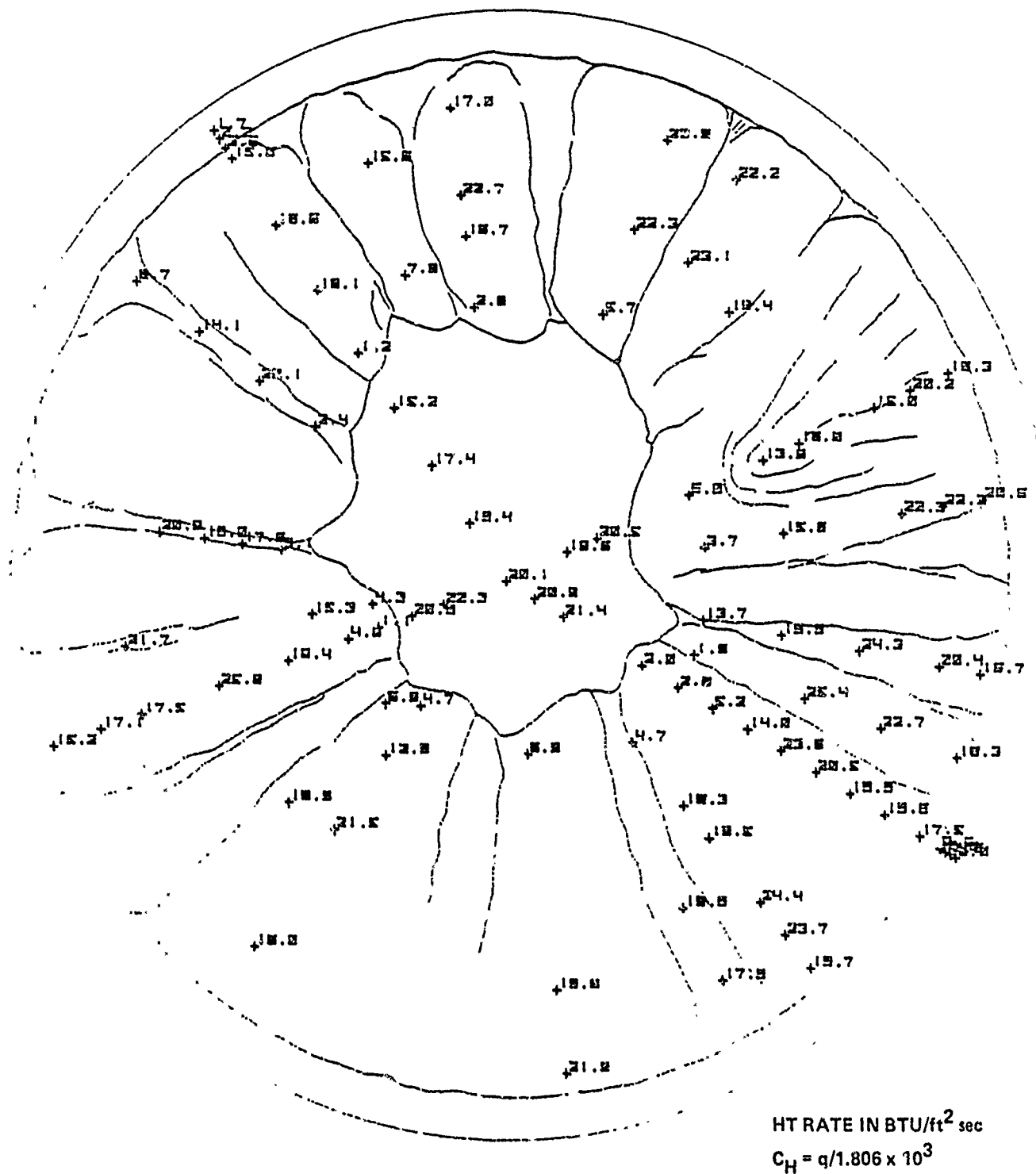
Figure 19a HEAT TRANSFER DISTRIBUTION OVER THE NRV CONFIGURATION – M = 11, Re/FT = 1 \times 10^6 , \alpha = 0^\circ
