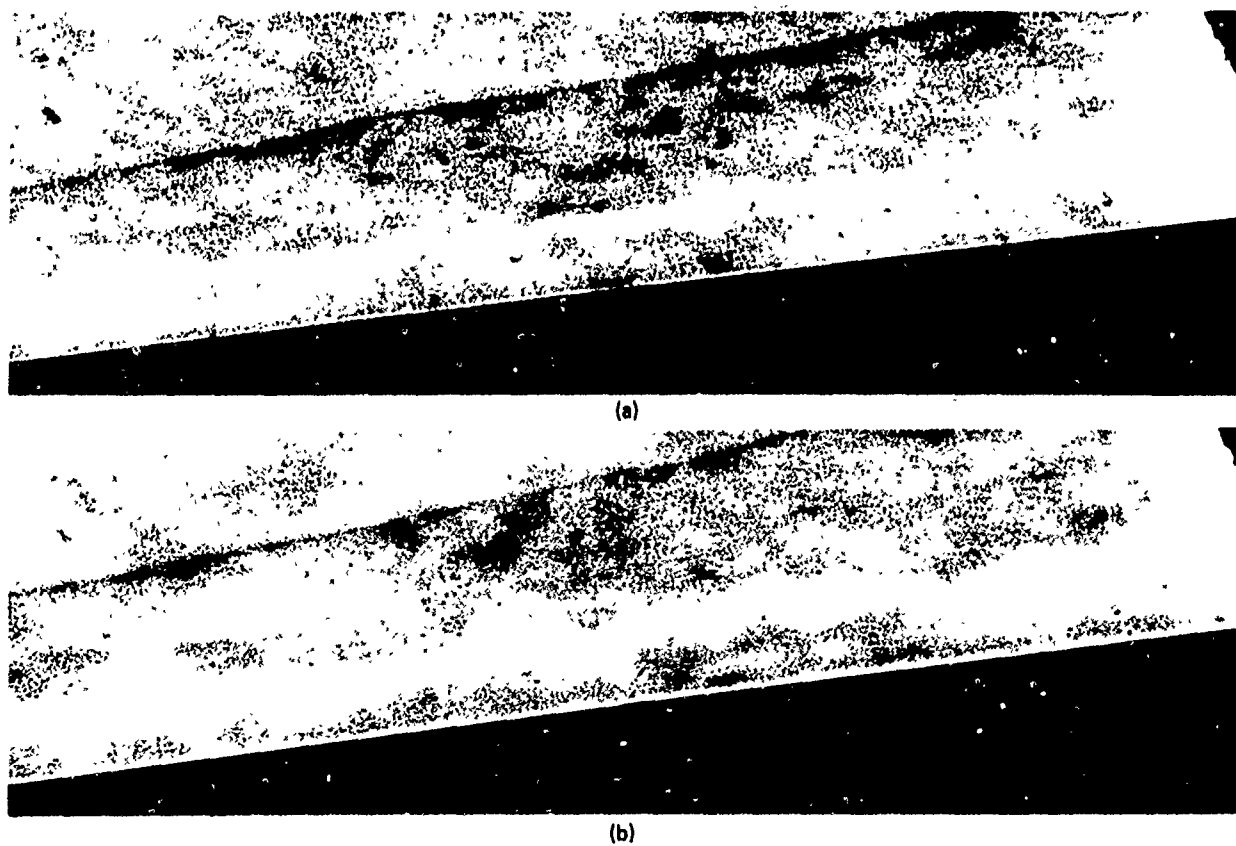
Figure 26 Schlieren Photographs of Gross-Instability Region (Ref. 57)
