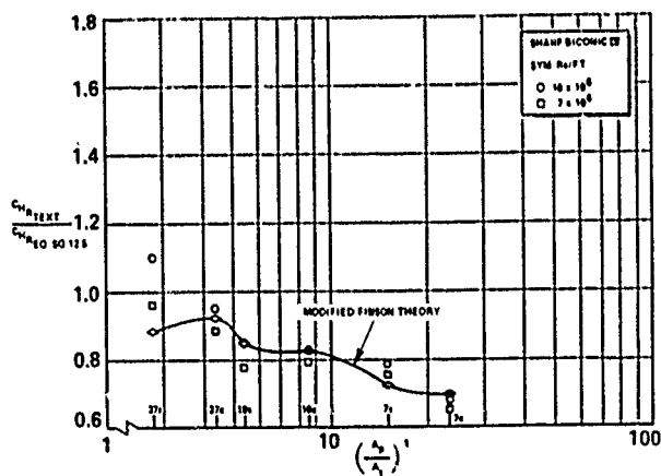
Figure 43 Correlation of Effective Roughness Heating Parameter For Sharp Biconic Nostips in Terms of the Effective Windward Area Parameter ( A_p/A_s )
