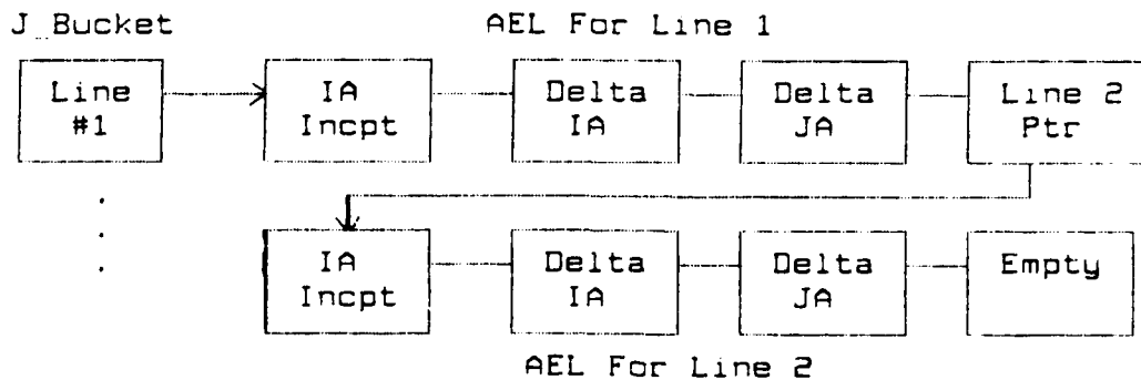
Fig. 3.6 Active Edge List Storage
