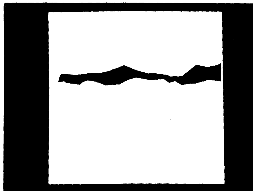
Fig 3.11 Synthesized Image 1
