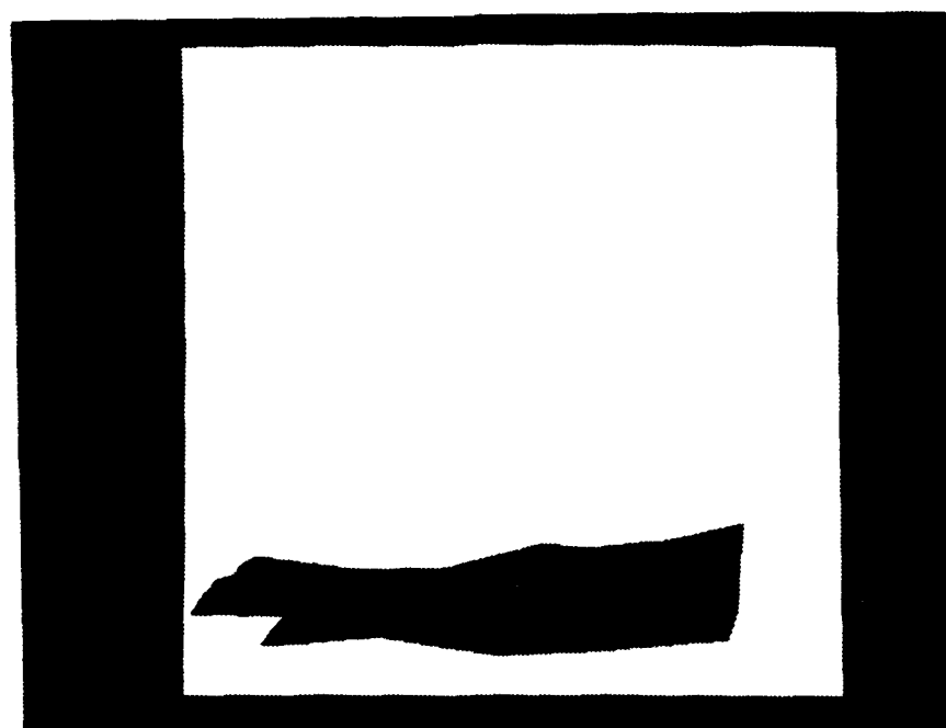
Fig. 3.12 Synthesized Image 2
