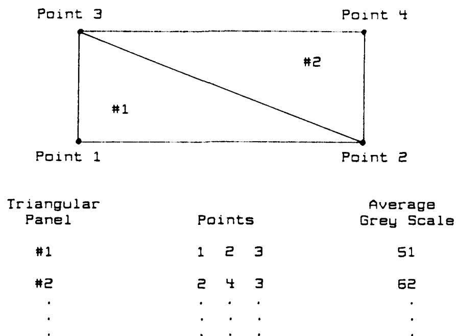
Fig. 3.5 Triangular Panel Data File Structure
