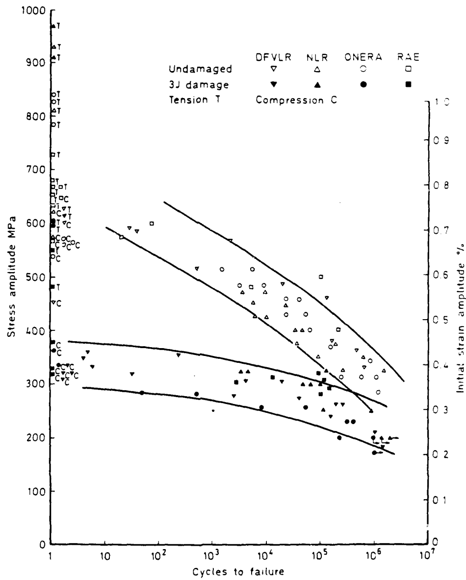
Fig 21 Combined fatigue results ( R = -1 ) from the four laboratories for undamaged and impact damaged [0\ 90\ 0\ \pm 45\ 0]_s carbon fibre laminates
