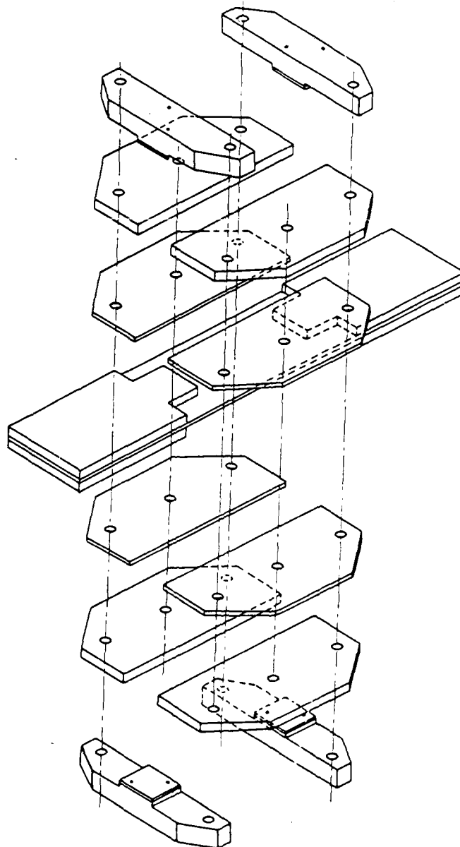
Fig 11 Exploded view of DFVLR anti-buckling device
