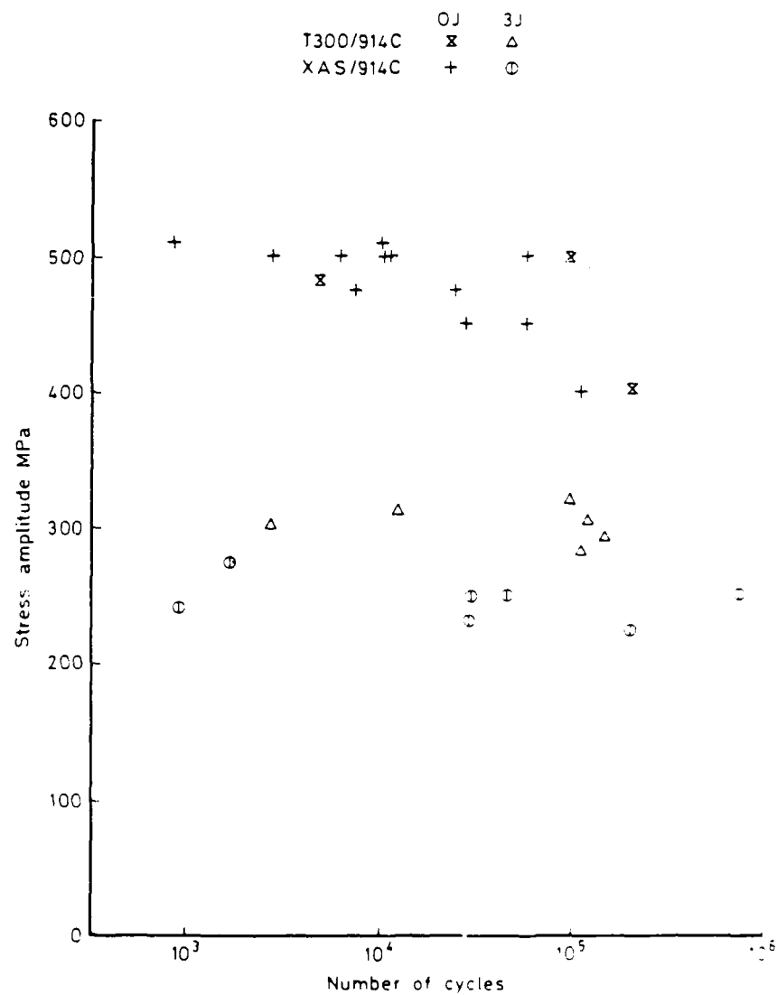
Fig 17 Fatigue curves ( R = -1 ) for undamaged and impact damaged [0\ 90\ 0\ \pm 45\ 0]_s carbon fibre laminates (RAE)
