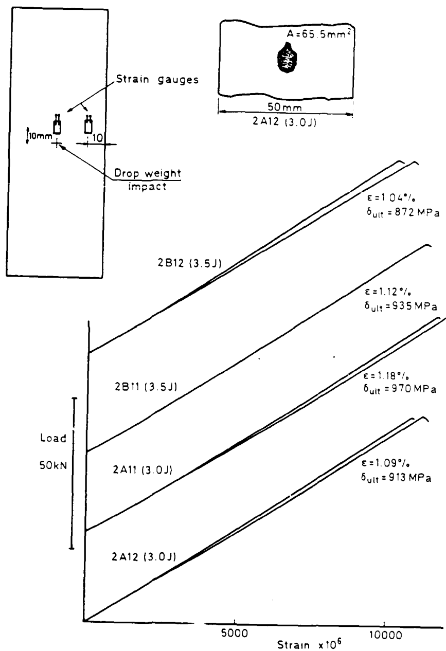
Fig 15 Load-strain curves of impact damaged specimens tested in tension and a typical C-scan of the damage (NLR)
