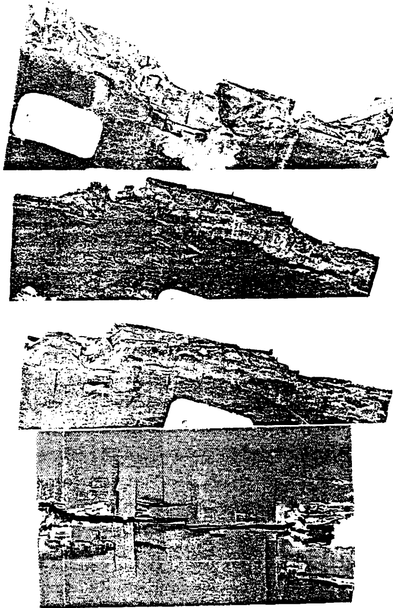
Fig 30 Fracture surfaces from non-impacted [0\ 90\ 0\ \pm 45\ 0]_s carbon fibre laminates tested in tension/compression fatigue (DFVLR)
