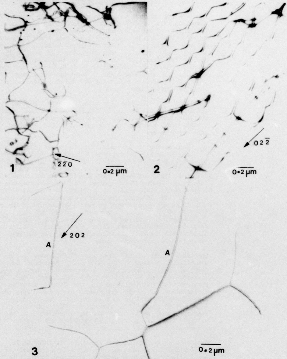
FIG. 1.--Bright field image , g[\bar{2}\bar{2}0] , foil orientation [001] . FIG. 2.--Bright field image showing hexagonal network of dislocations, g[02\bar{2}] , foil orientation [011] . FIG. 3.--Bright field image, g[202] and foil orientation [\bar{1}11] .
