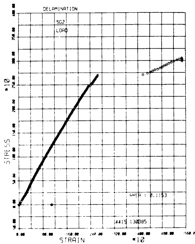
(c) Transverse Gage 2
