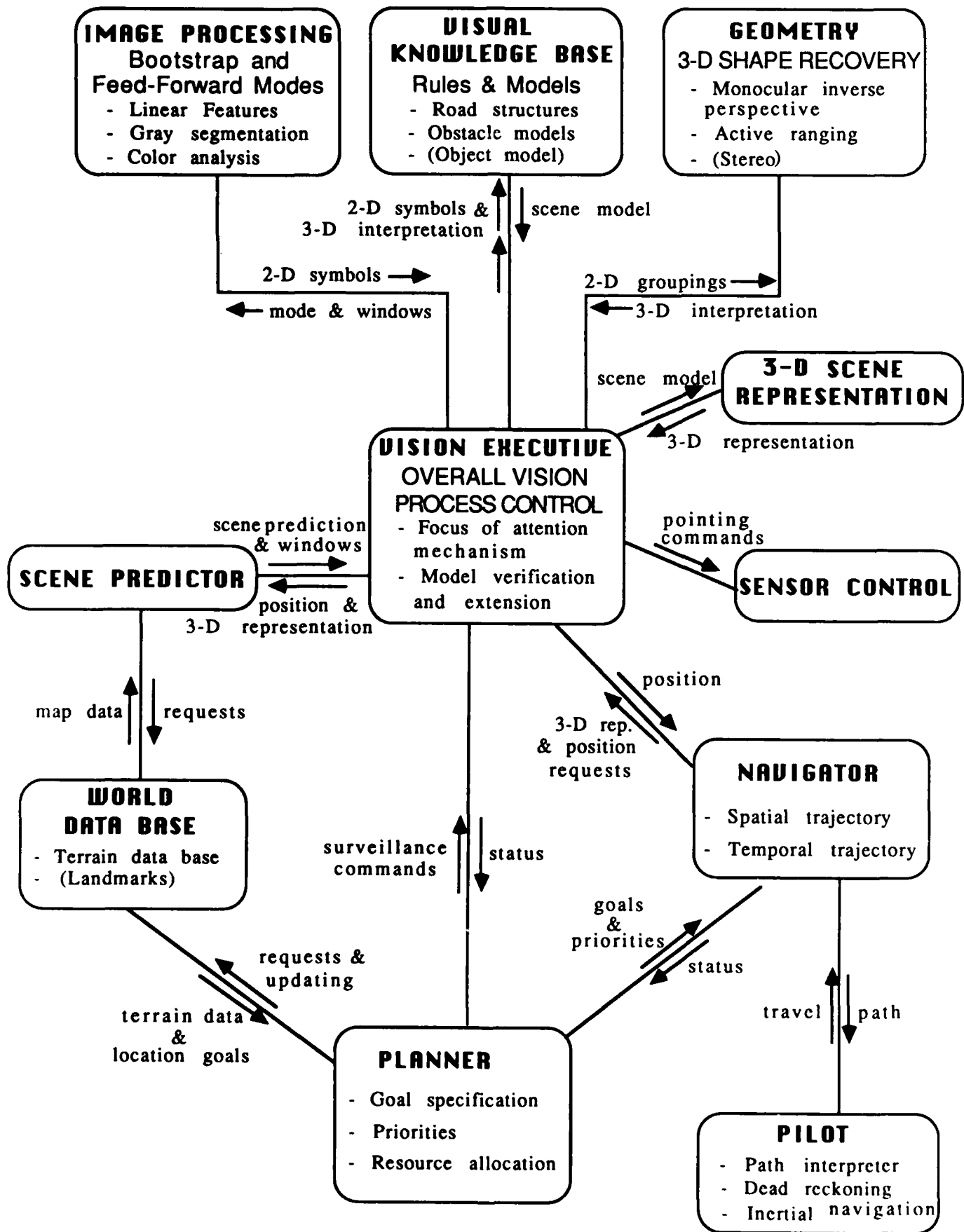
Figure 1.1 System configuration
