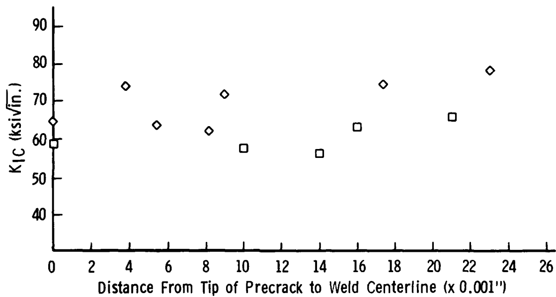
Figure 7. Fracture toughness values plotted vs. the distance from the tip of the precrack to the weld centerline for 0.004% sulfur (□) and 0.014% sulfur (◇) materials.
