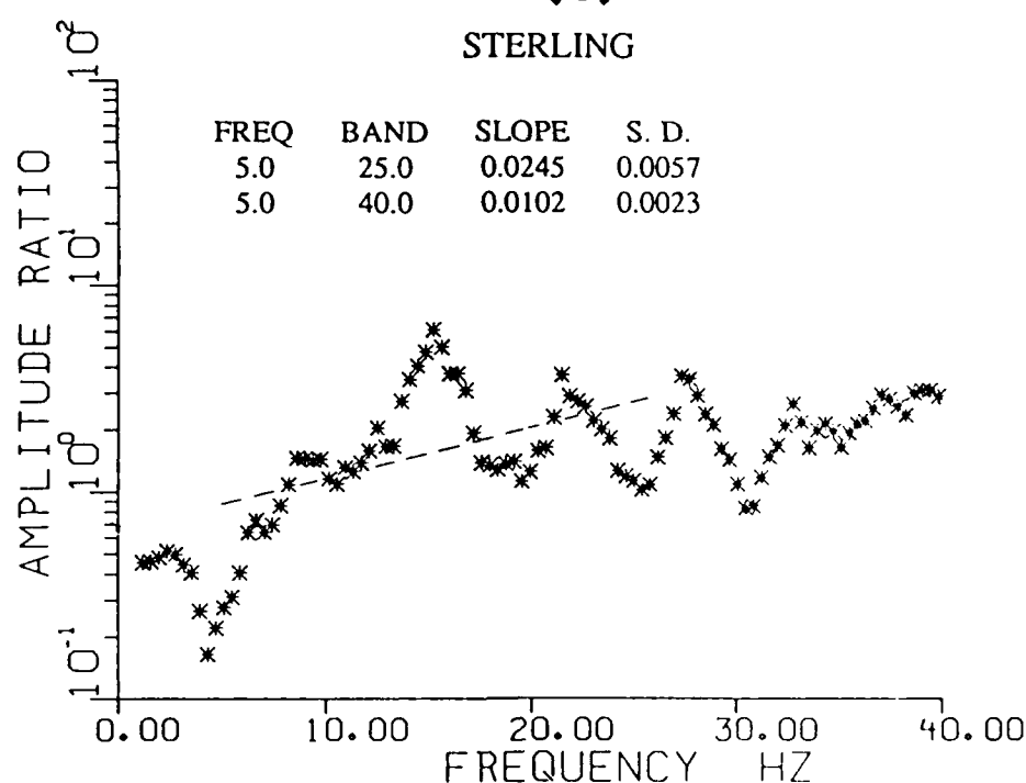
Figure 13. Spectral ratio P/Lg, corrected for noise, for (a) Salmon and (b) Sterling recorded at station PL-MS. Points for which S/N power ratio is less than 2 are not plotted. The dashed lines show mean (least squares) slopes over the frequency range 5 to 25 Hz. The mean value of slope/Hz and its standard deviation (S.D.) are indicated for frequency ranges of 5 to 25 and 5 to 40 Hz.
