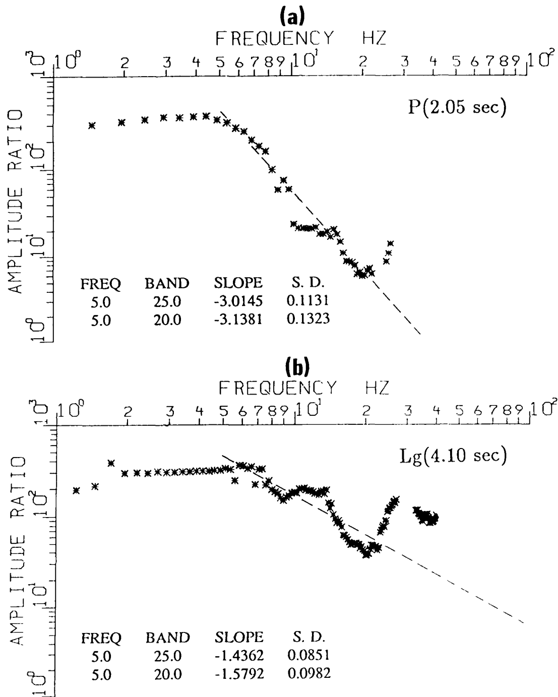
Figure 11. Spectral ratio Salmon/Sterling, corrected for noise, with logarithmic frequency scale, for (a) P window 2.05 sec long, and (b) Lg window 4.10 sec long, recorded at station 20S. The dashed lines show mean (least squares) slopes over the frequency range 5 to 25 Hz. The mean value of slope and its standard deviation (S.D.) are indicated for frequency ranges of 5 to 25 and 5 to 20 Hz.
