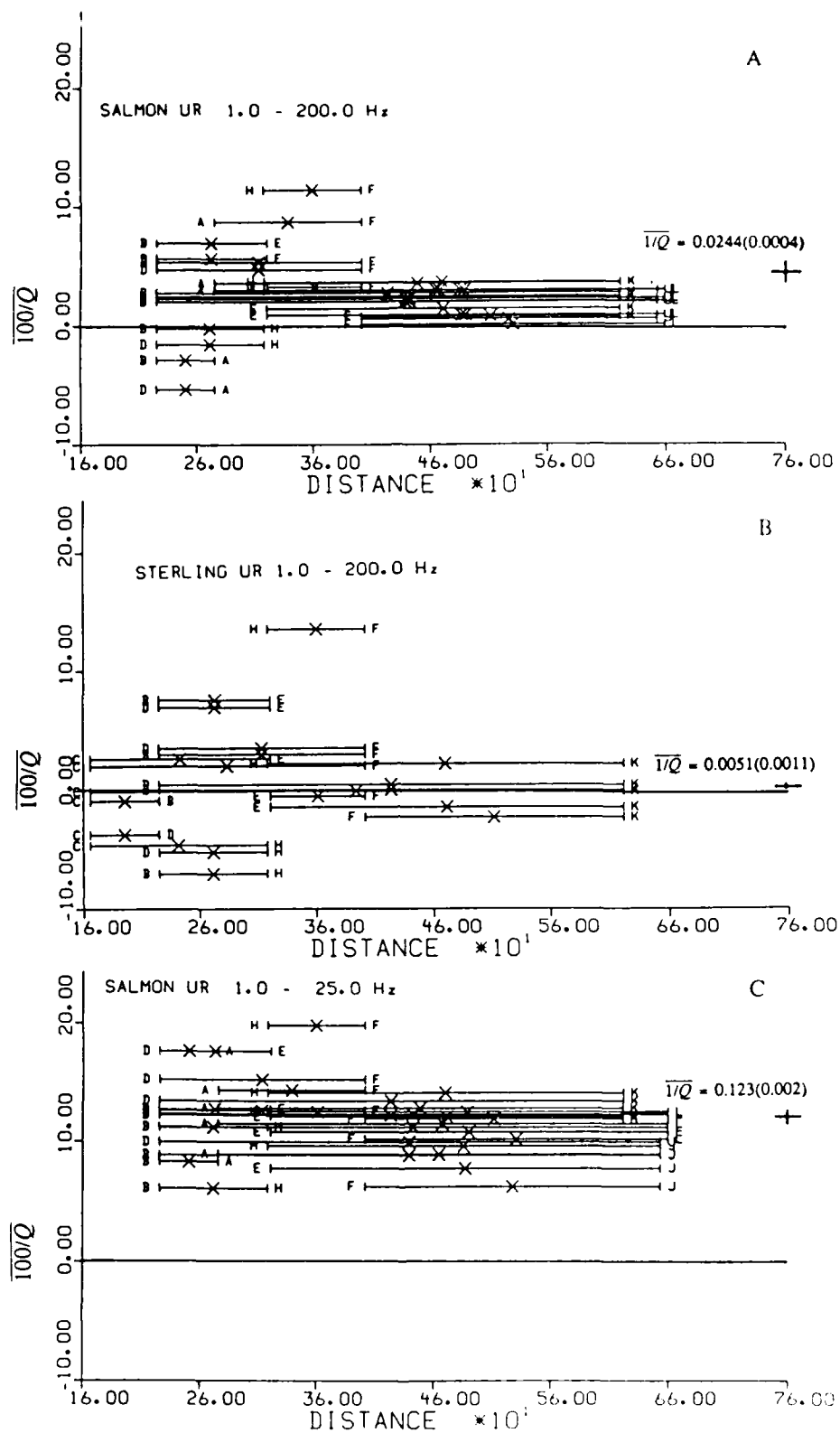
Figure 6. (6A) \overline{1/Q} estimates for Salmon in the 1-200 Hz bandwidth from the URH sensor pairs. Mean \overline{1/Q} = 0.0244(0.0004) , or \overline{Q} = 40.9(0.7) . (6B) \overline{1/Q} estimates for Sterling in the 1-200 Hz bandwidth from the URH sensor pairs. Mean \overline{1/Q} = 0.0051(0.0011) or \overline{Q} = 196(40) . (6C) \overline{1/Q} estimates for Salmon in the 1-25 Hz bandwidth from the URH sensor pairs. Mean \overline{1/Q} = 0.123(0.002) , or \overline{Q} = 8.1(0.1) .
