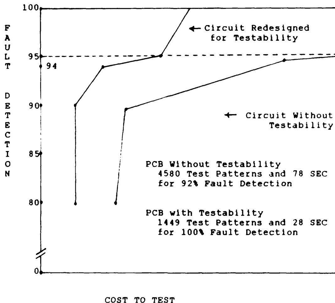
Fig 1. Cost-to-Test of a Printed Circuit Board
