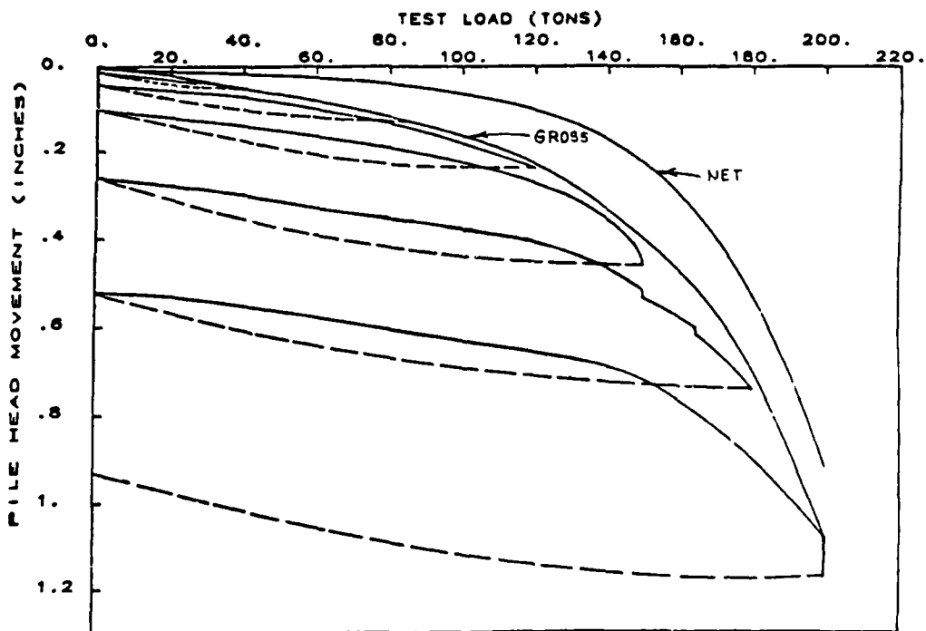
Figure B6. Pile Test 3B, compression
