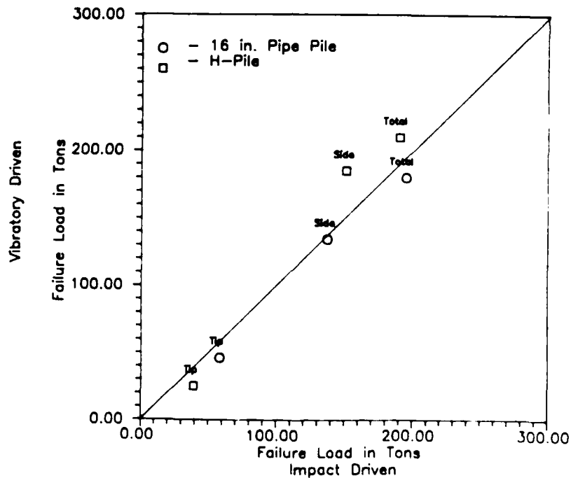
Figure 18. Comparison of load distribution of impact- and vibratory-driven piles for Look and Lam No. 4
