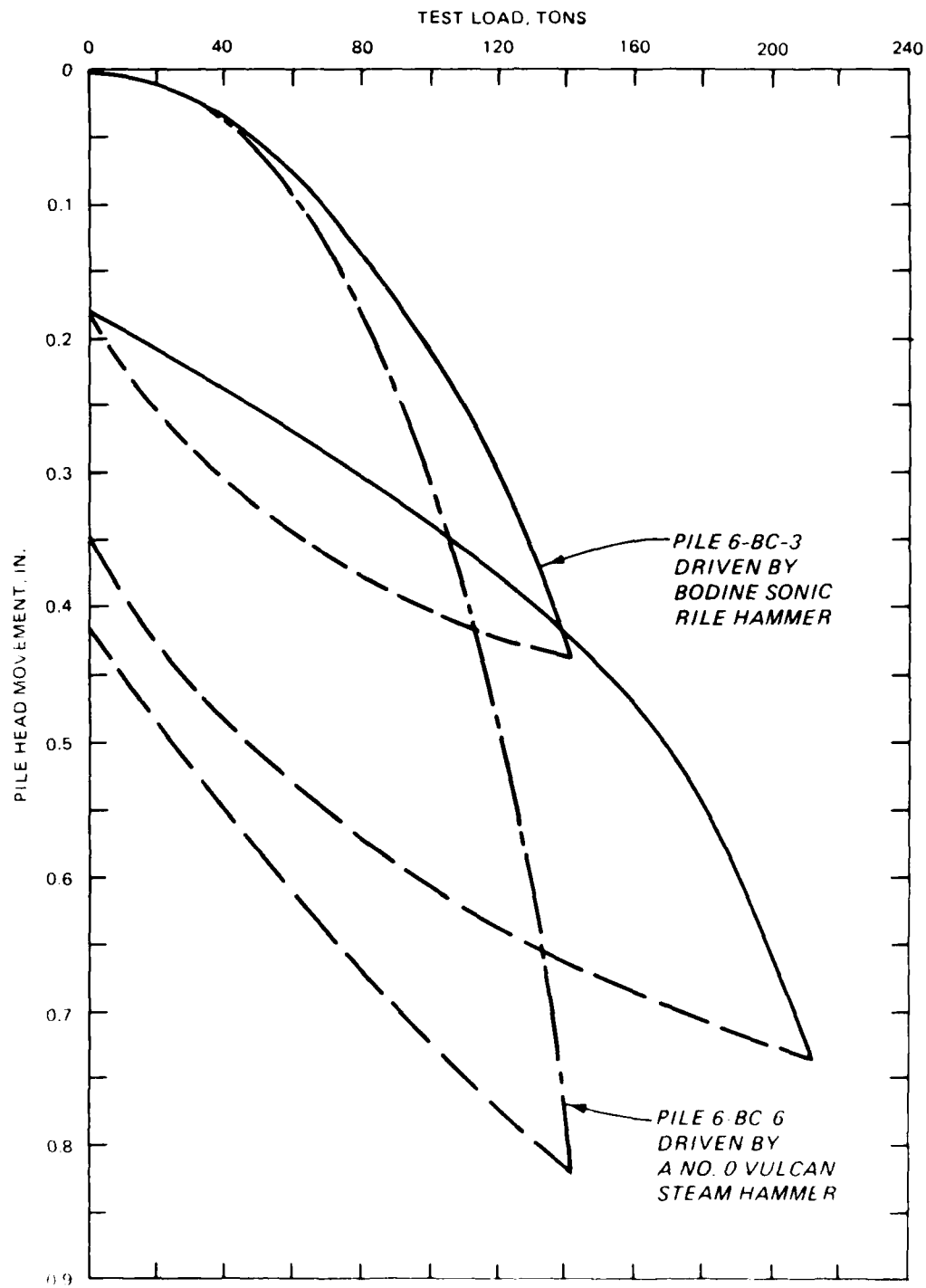
Figure 15. Pile load tests for Geophysical Building
