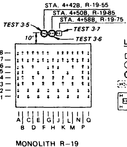
Figure 5. Location of pile tests (Continued)
