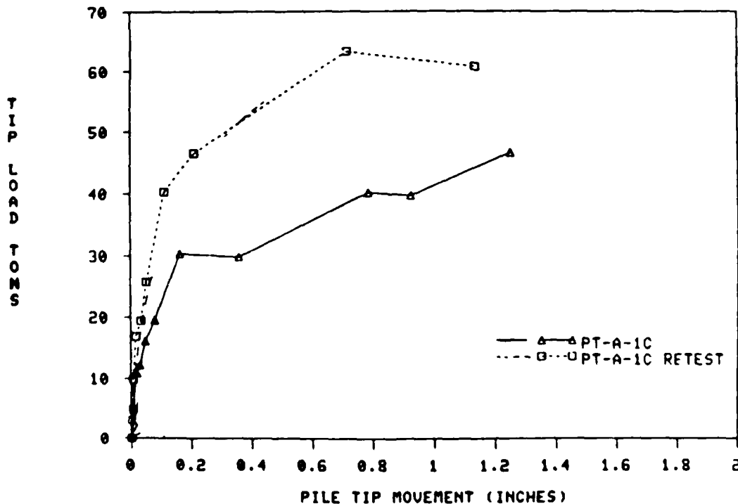
Figure 19. Tip load versus pile tip movement for Pile A-1C, Red River Lock and Dam No. 1 (Mosher 1984)
