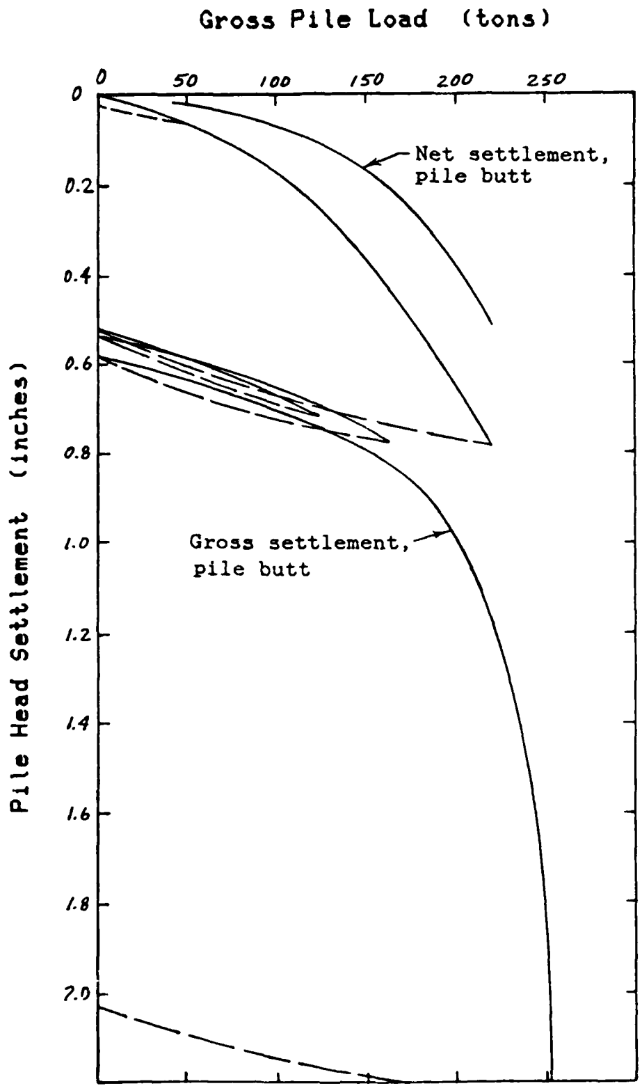
Figure A8. Compression test results - Test Pile 7 (14 BP 73)
