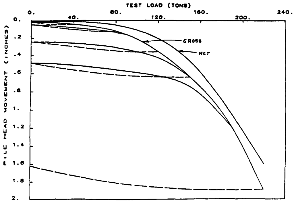
Figure B9. Test Pile 9, compression
