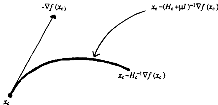
Figure 4.3.1 The trust region curve
