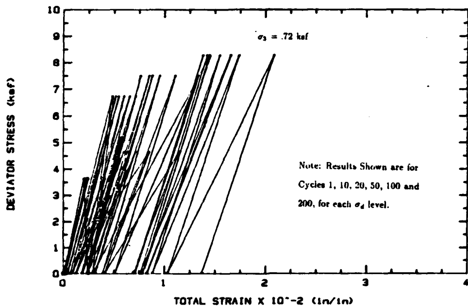
San Antonio Airport 5' Cyclic Triaxial Test Results
