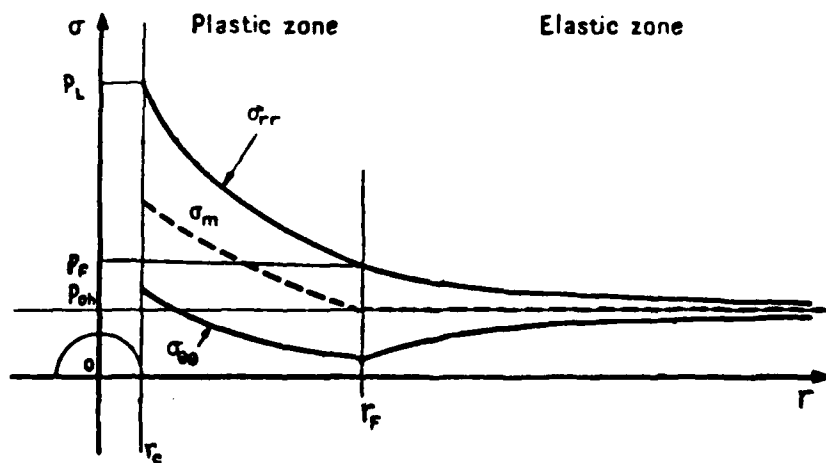
Fig. F2 Stresses in Elastic-Plastic Soil (from Baguelin et al. 1978)
