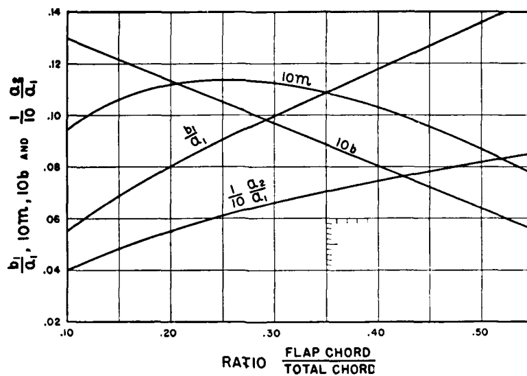
Figure 60. Theoretical Flap Relations
