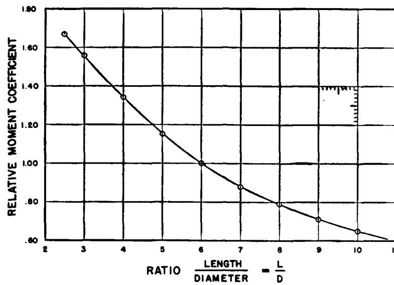
Figure 97. Effect of Fineness Ratio on Yawing Moment Coefficient
