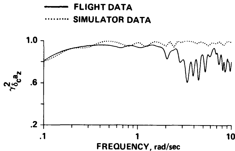
Fig. 4.28. Coherence Function for Vertical-Acceleration Response Identification ( \gamma_{\delta a_z}^2 ).
