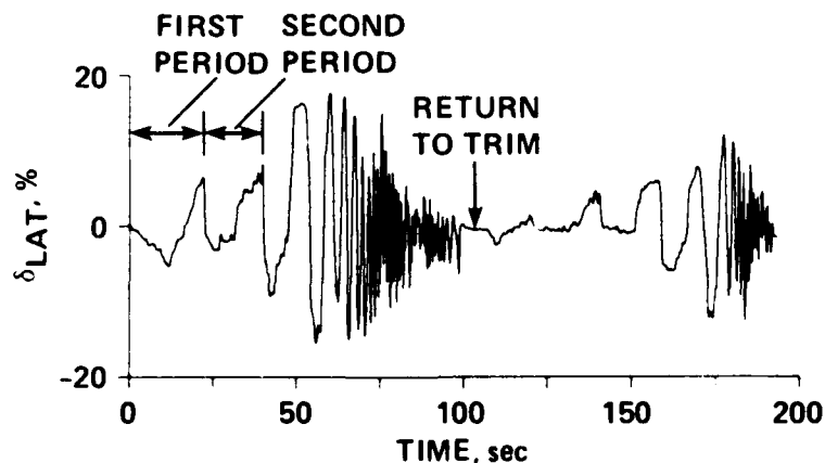
Fig. 4.1. Two Lateral-Stick Frequency-Sweeps ( \delta_{LAT} ) in Hover.
