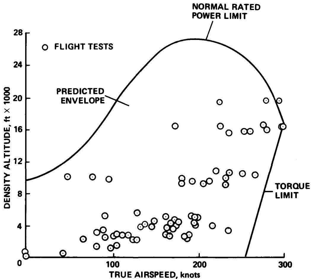
Fig. 2.2. Airspeed-Altitude Envelope.
