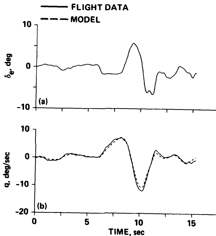
Fig. 4.35. Pitch-Response Model Verification Using SCAS-off Flight Data. (a) Elevator Input; (b) Pitch-Rate.
