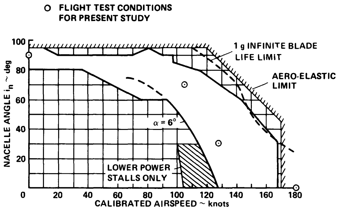
Fig. 2.3. Conversion Corridor.
