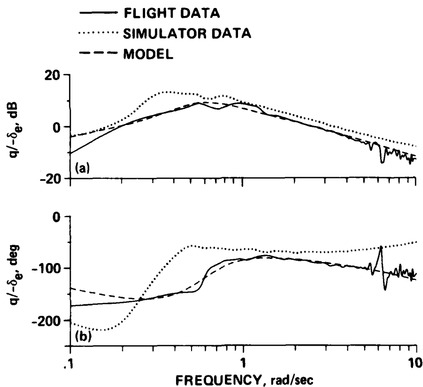
Fig. 4.29. Pitch-Rate Response to Elevator ( q/-\delta_e ).
