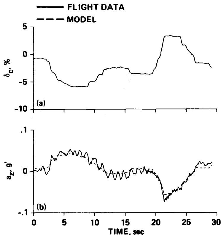
Fig. 4.34. Vertical-Acceleration Response Model Verification.
