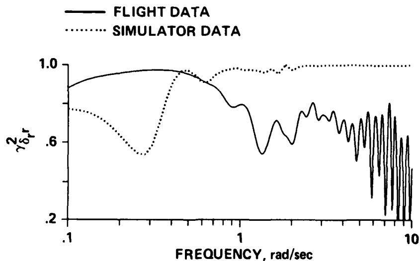
Fig. 4.12. Coherence Function for Yaw-Rate Response Identification ( \gamma^2_{\delta_{\dot{r}}r} ).
