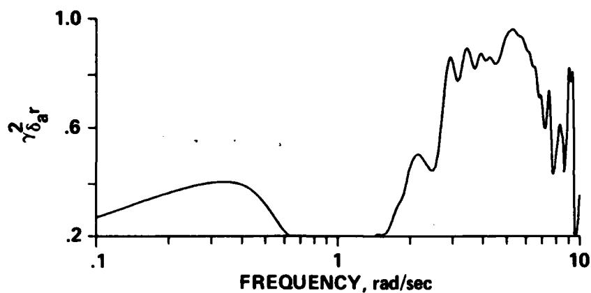
Fig. 4.21. Coherence Function for Yaw-Rate Response to Aileron Inputs ( \gamma_{\delta_r}^2 ).
