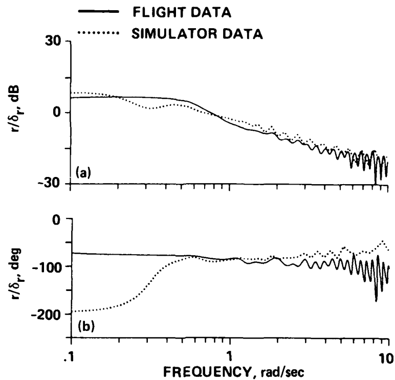
Fig. 4.11. Yaw-Rate Response to Rudder ( r/\delta_{\dot{r}} ). (a) Magnitude; (b) Phase.
