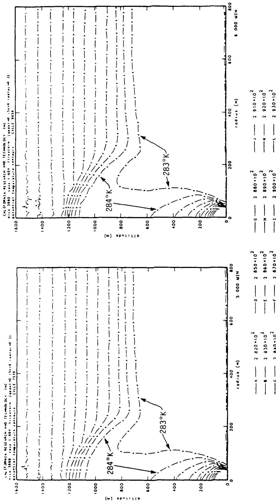
Figure 39e. Model potential temperature field at 5 minutes into the Meteoron simulation run. Contour interval is 1°K.
