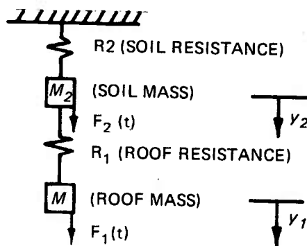
Figure 1. Degree-of-freedom models
