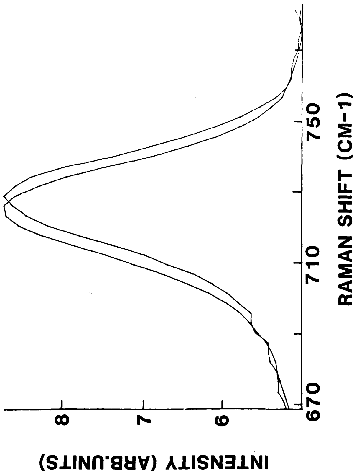
Figure 6. Raman Spectra of the \nu_4 ( E' ) Mode of \text{NO}_3^- Taken for 13 M Aqueous HAN. The spectrum to the left (lowest frequency peak) is for a temperature of 22°C; the other a temperature of -50°C.
