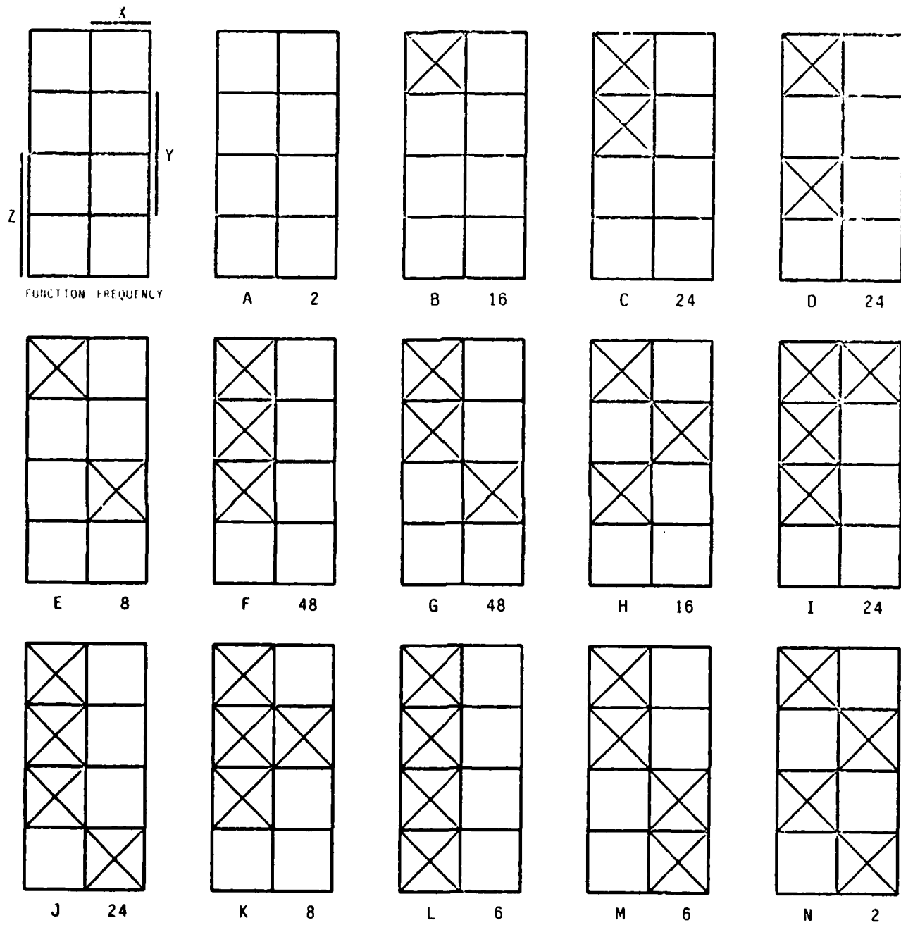
Figure 4-1: Unique Boolean Functions of 3 Inputs
