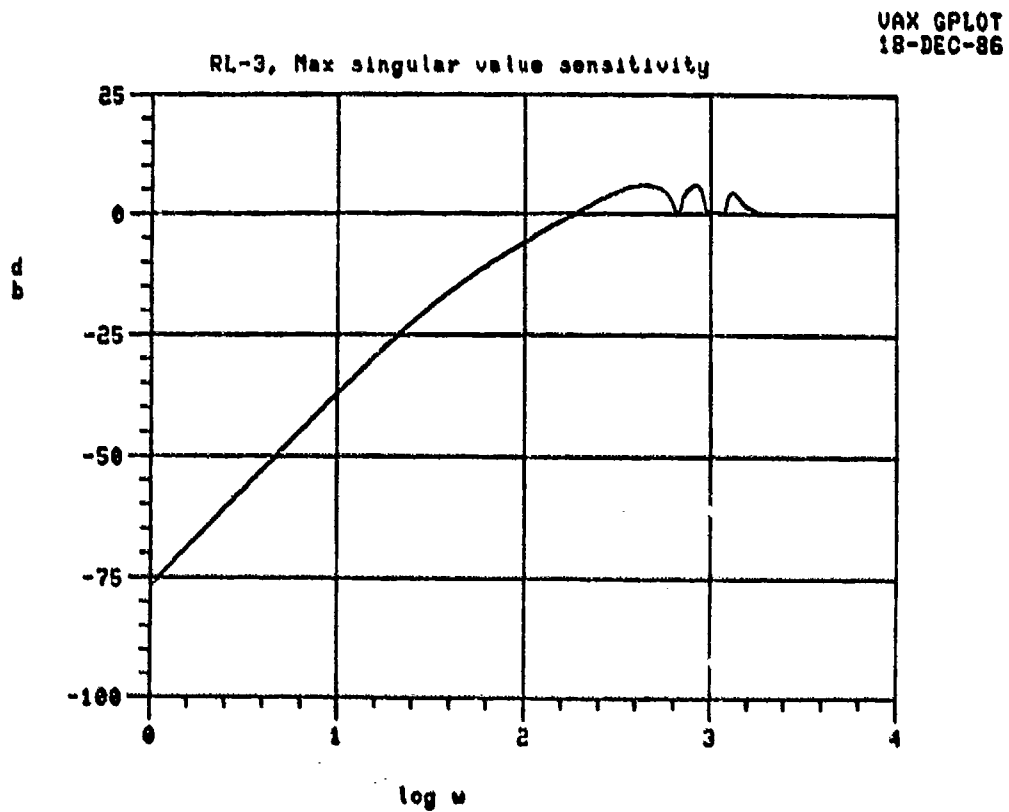
Fig. 15b: RL-3 maximum singular value sensitivity function
