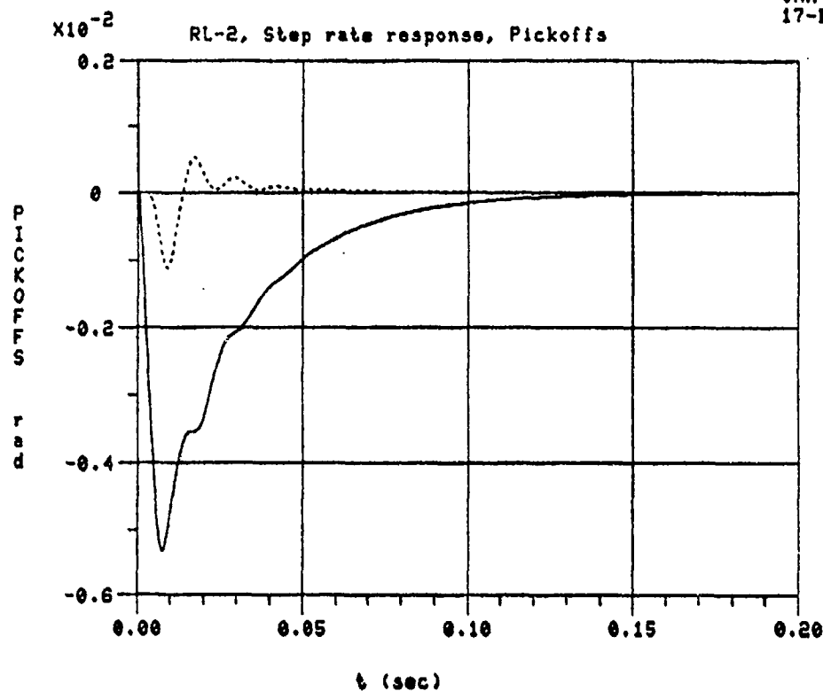
Fig. 5a: RL-2 step rate response (pickoffs); — \theta_x , --- \theta_y
