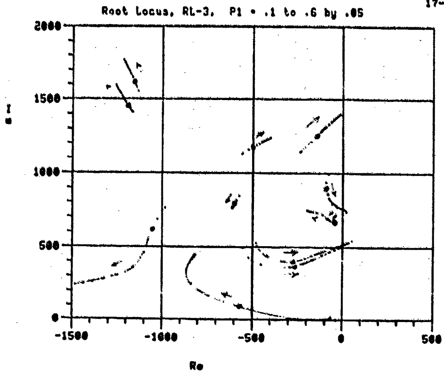
Fig. 2b: RL-3 root Locus varying p_1
