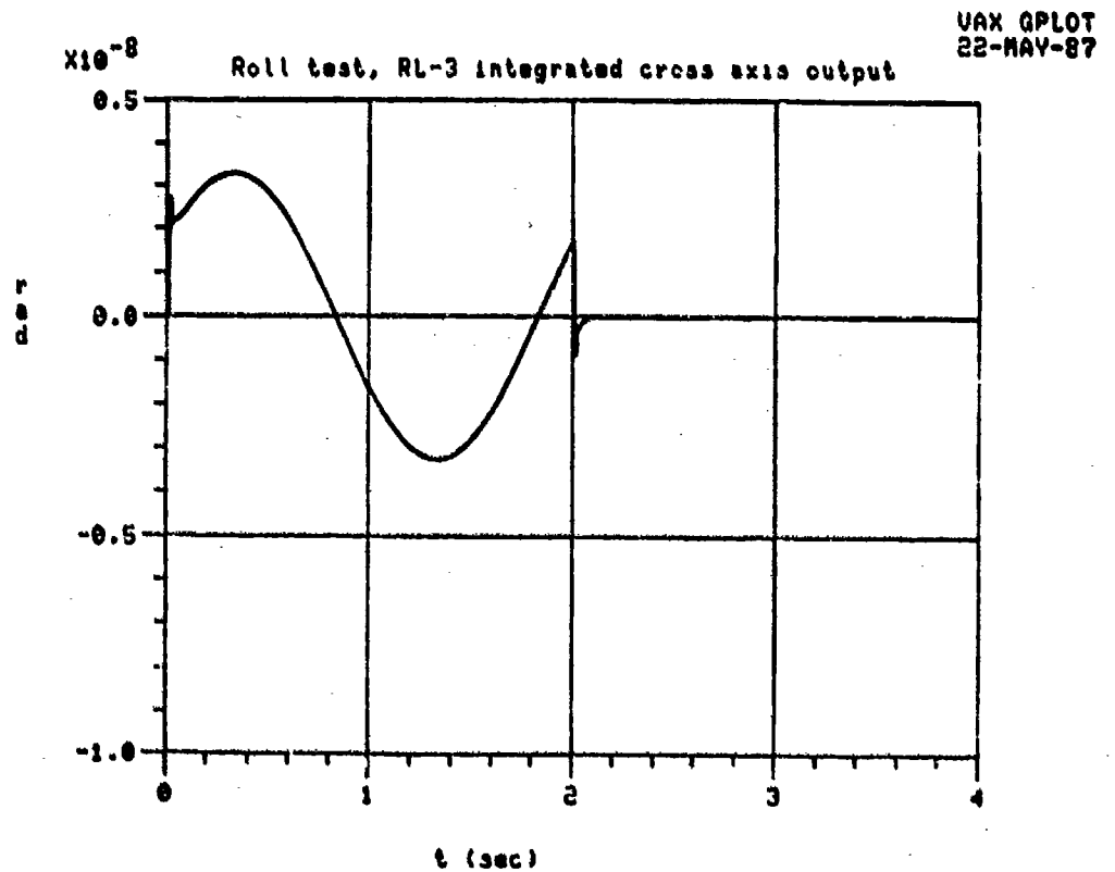
Fig. 12b: RL-3 roll test, integrated cross-axis output = \int OUT_y
