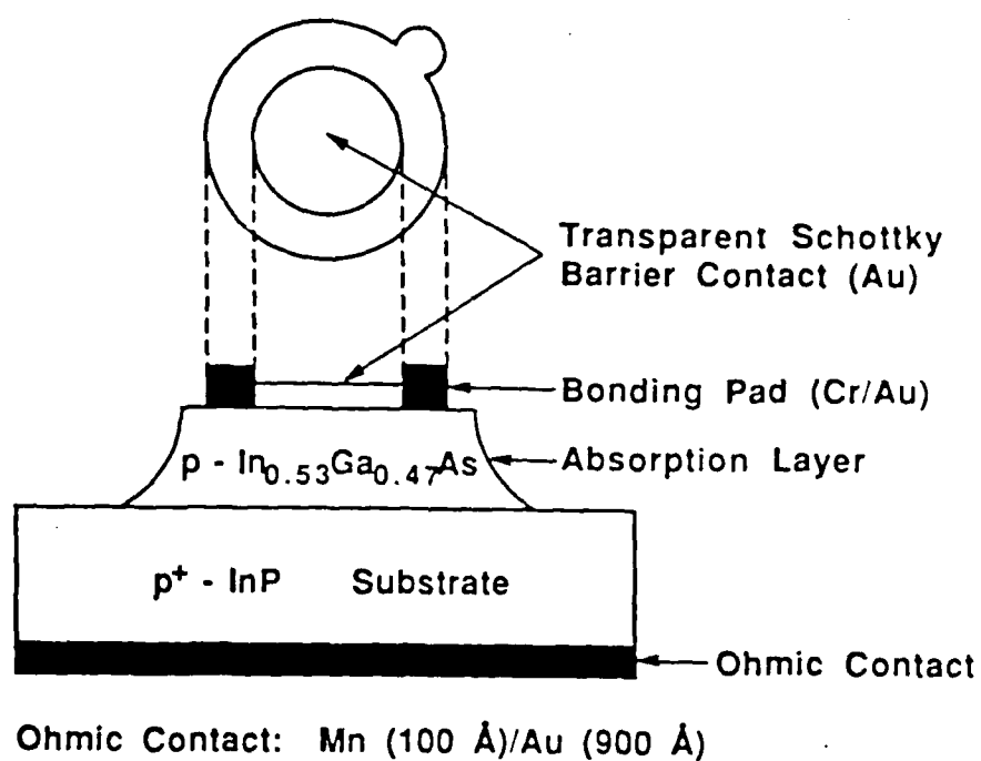
Fig. 3.5. Structure of p\text{-InGaAs}/p^+\text{-InP} Schottky Barrier Diode.
