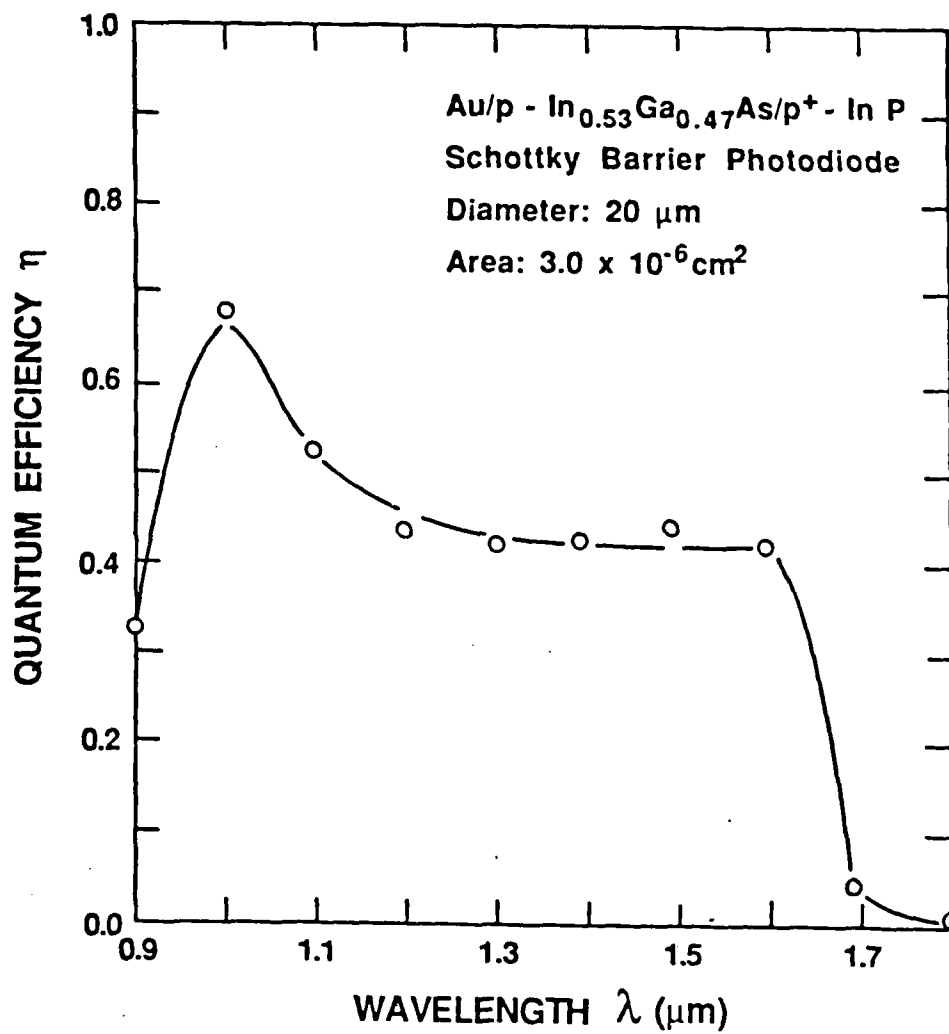
Fig. 5.9. Quantum Efficiency of p-InGaAs/p + -InP Schottky Barrier Photodiode.
