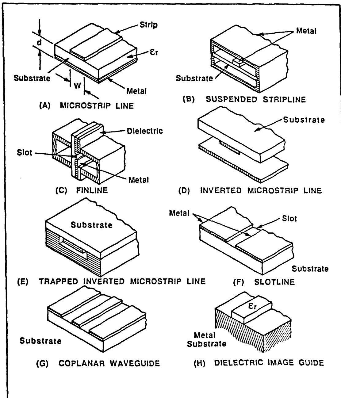
Fig. 2.4. Structure of Microwave Package for MIC Applications
