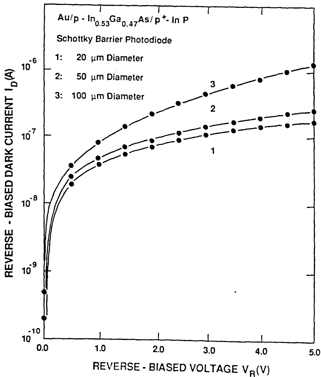
Fig. 5.5. Reverse-biased Dark Current of p-InGaAs/p + -InP Schottky Barrier Photodiode.
