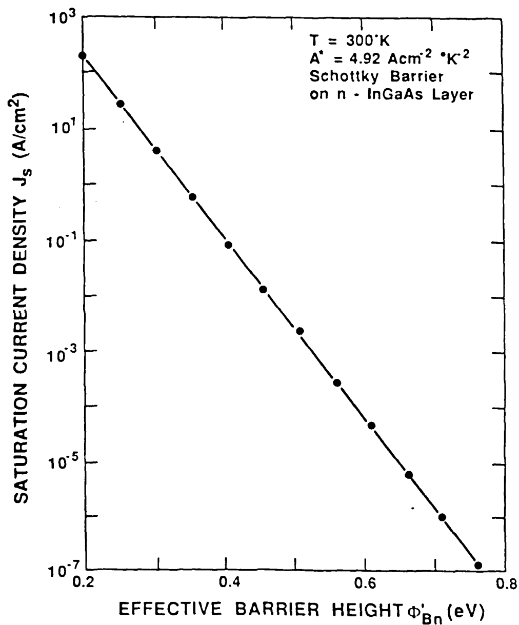
Fig. 3.3. Theoretical Saturation Current Density vs. Effective Barrier Height.
