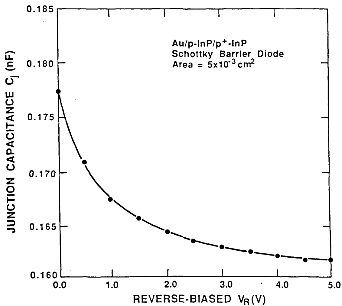
Fig. 3.14. Junction Capacitance of p-InP/p + -InP Schottky Barrier Diode.
