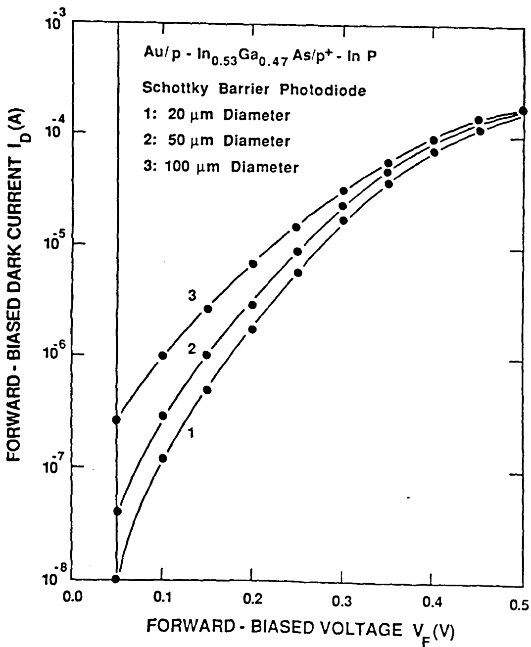
Fig. 5.4. Forward-biased Dark Current of p-InGaAs/p + -InP Schottky Barrier Photodiode.
