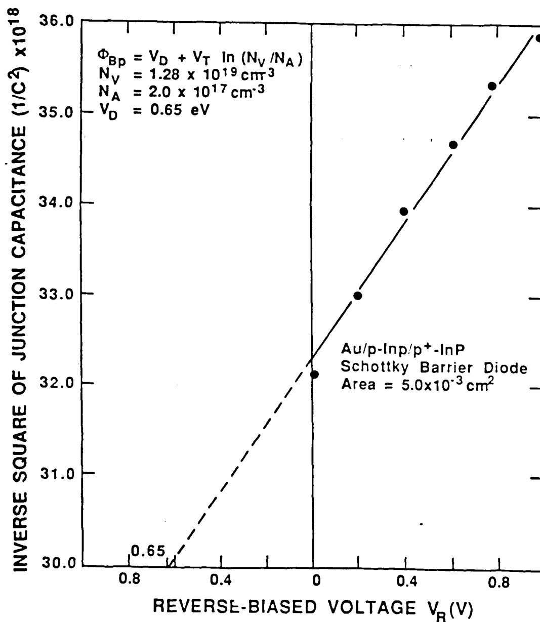
Fig. 3.15. Inverse Square of Junction Capacitance of p-InP/p + -InP Schottky Barrier Diode.
