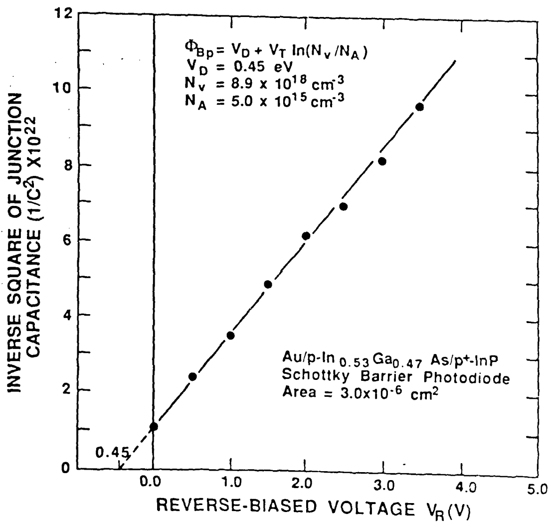
Fig. 5.6. Inverse Square of Capacitance of p-InGaAs/p + -InP Schottky Barrier Photodiode.
