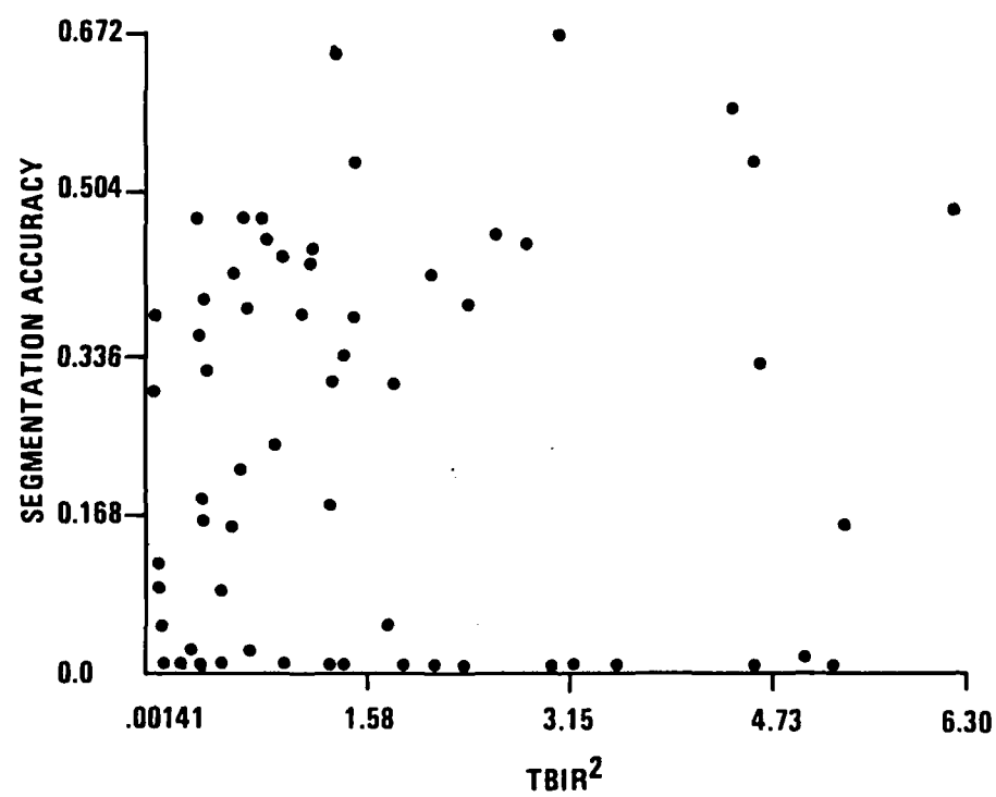
Figure 4-11. Variation of Segmentation Accuracy as TBIR^2 Varies for 28 Frames from 29-Palm Data Base
