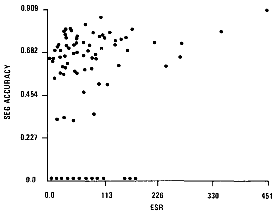
Figure 3-45. Variations of Segmentation Accuracy as ESR Varies for Sequence 5 of the Honeywell MSN1712 Data Base
