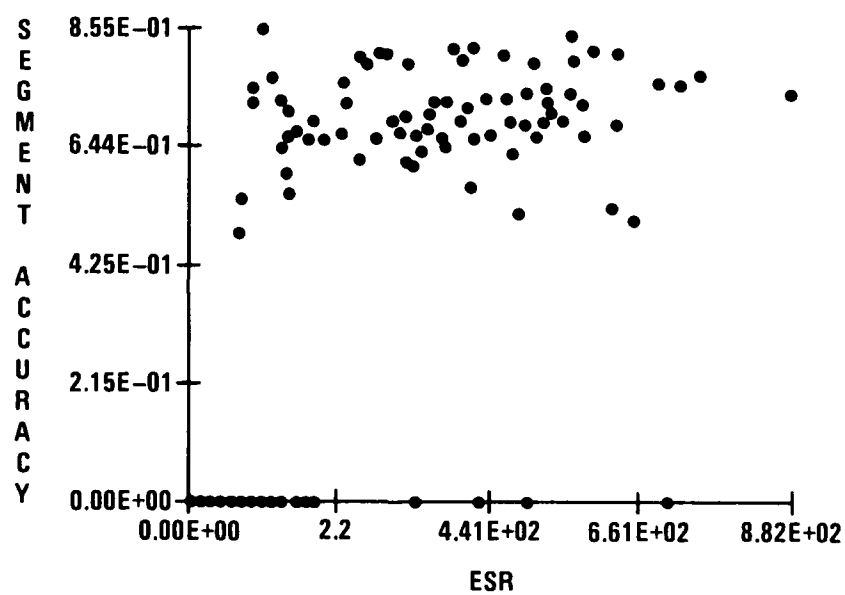
Figure 3-33. Segmentation Accuracy as a Function of ESR (sequence 1)
