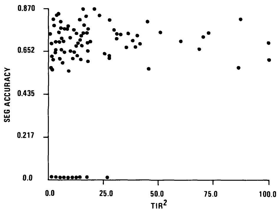
Figure 3-40. Variations of Segmentation Accuracy as TIR 2 Varies for Sequence 4 of the Honeywell MSN1712 Data Base
