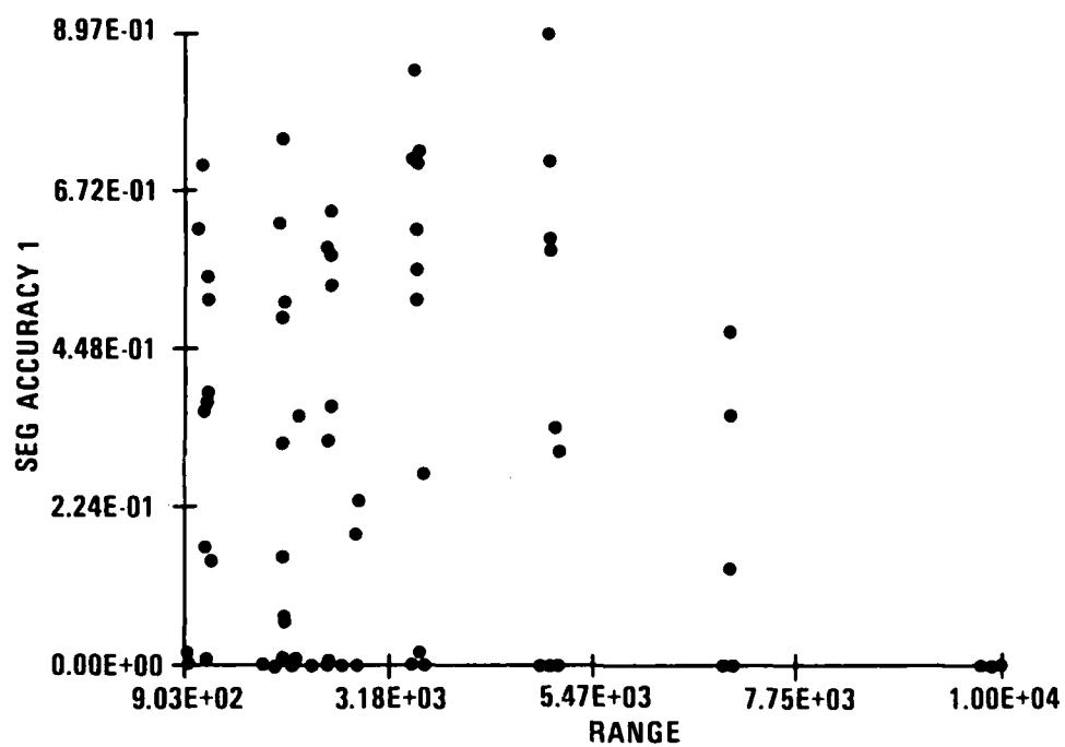
Figure 4-22. Variation of Segmentation Accuracy as a Function of Range for the T3002 Data Base
