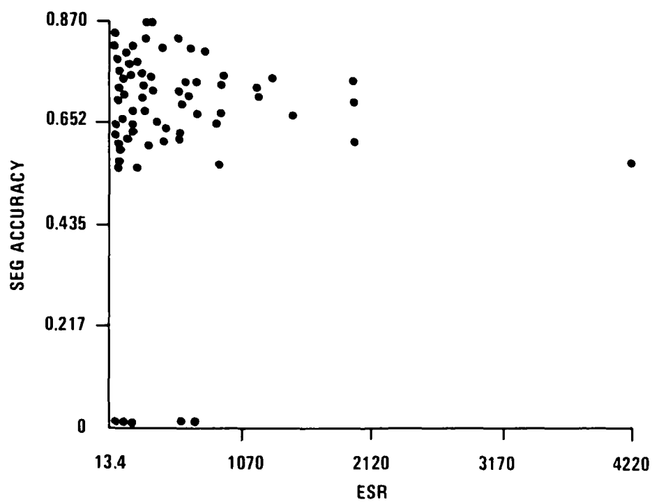
Figure 3-42. Variations of Segmentation Accuracy as ESR Varies for Sequence 4 of the Honeywell MSN1712 Data Base
