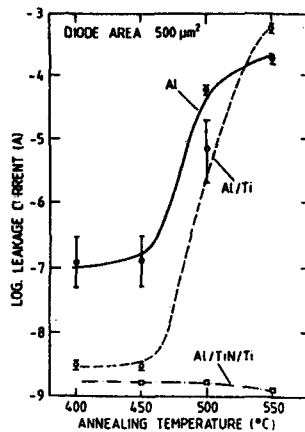
Fig.5 A successful application of the reactively sputtered refractory compound TiN as a thin-film diffusion barrier (from [8]). The figure shows the leakage current of a reverse biased Si n^+p junction with Al/Si, Al/Ti/Si and Al/TiN/Ti/Si contact systems as a function of the temperature of an annealing treatment in flowing argon for 15 min.
