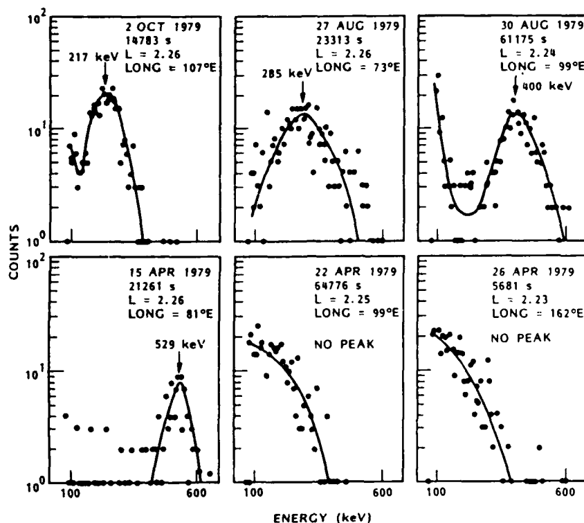
Fig. 2. Representative examples of the energy spectra of electrons observed in the drift loss cone from the P78-1 satellite. Best fit curves to the data points are shown.
