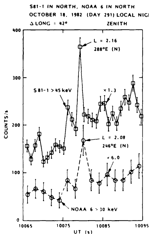
Fig. 7. An example of a coincident event observed in both the S81-1 and the NOAA 6 zenith instruments. The S81-1 points represent average counts per second in successive 1-s intervals, and these are interconnected by solid lines to indicate continuous coverage. The NOAA 6 points represent the counts recorded in alternate 1-s intervals and are interconnected by dashed lines to represent the 50% duty cycle for data coverage.
