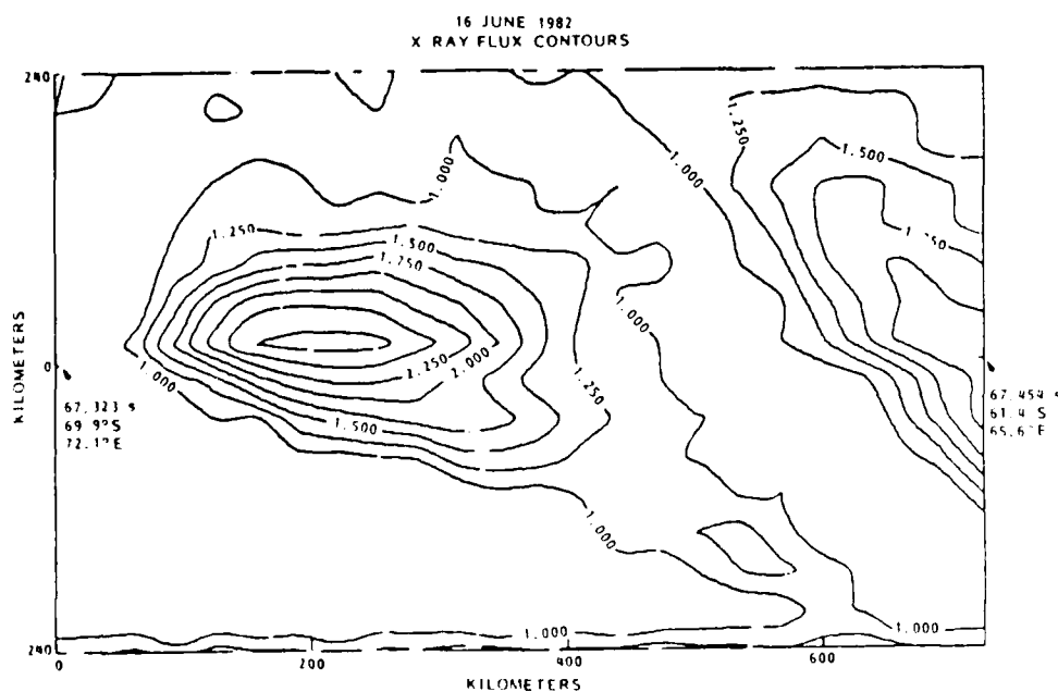
Fig. 5. Examples of the contour plots for an isolated small X ray patch and for an elongated patch. Corrections have been made for the projected dimensions with a flat earth approximation. The contours are labeled by the logarithm to the base 10 of the counts per second.
