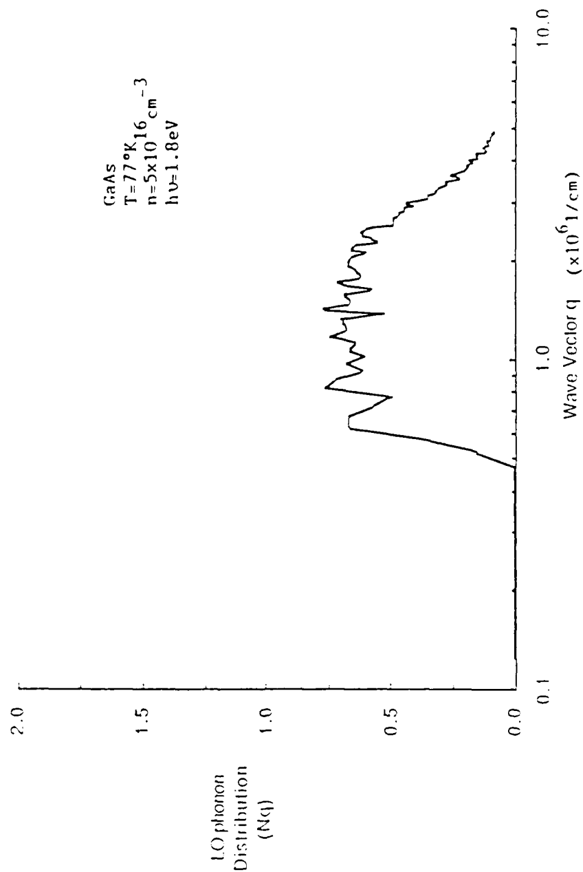
Fig. 4.8 The non equilibrium LO phonon occupation number versus phonon wave vector q at t=10 ps.
