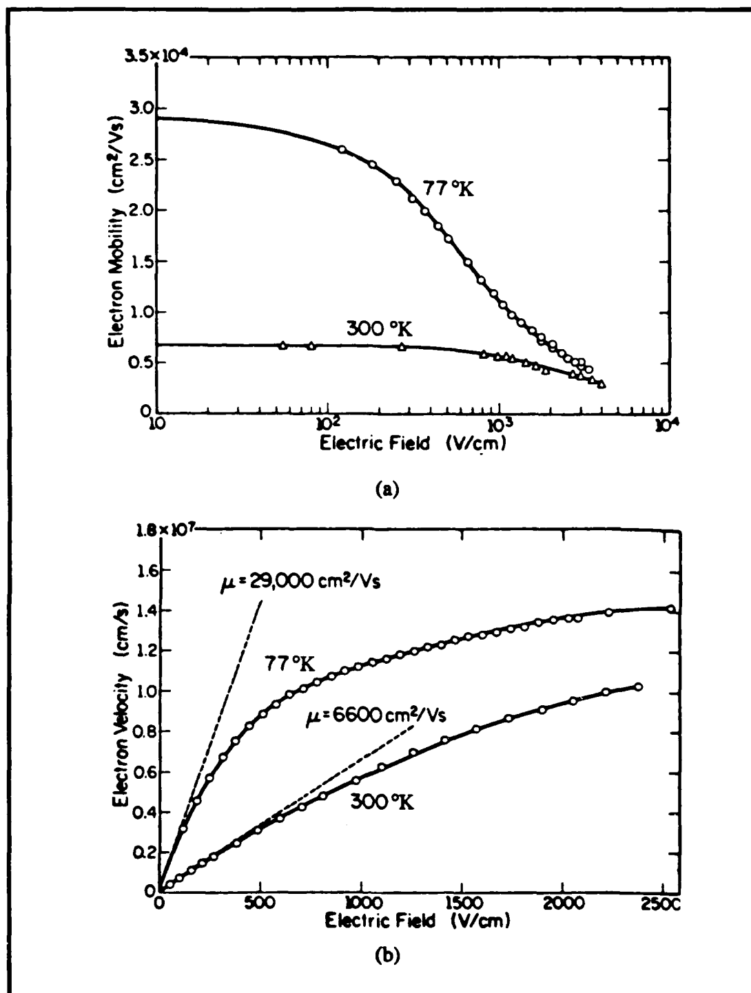
Fig. 2.19 (a) Electron Mobility and (b) Electron Velocity vs. Electric Field at 77 and 300 °K for an InGaAs/AlGaAs Pseudomorphic MODFET Structure [46:565]
