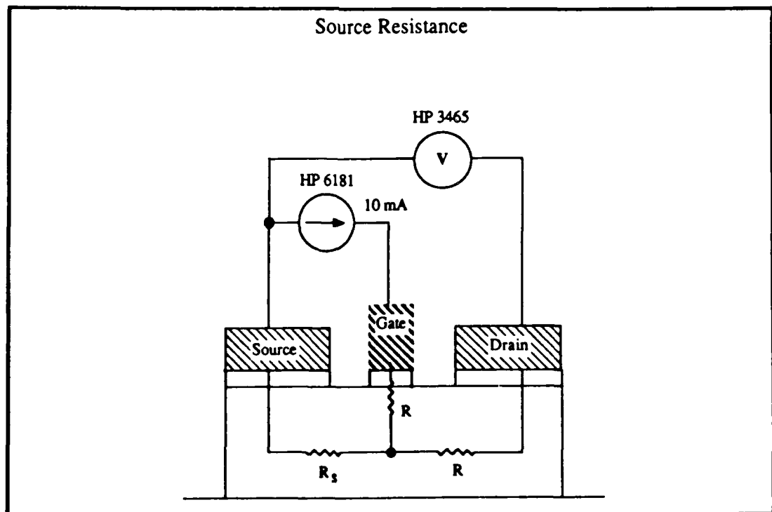
Fig. 4.7 Source Resistance Measurement Technique
