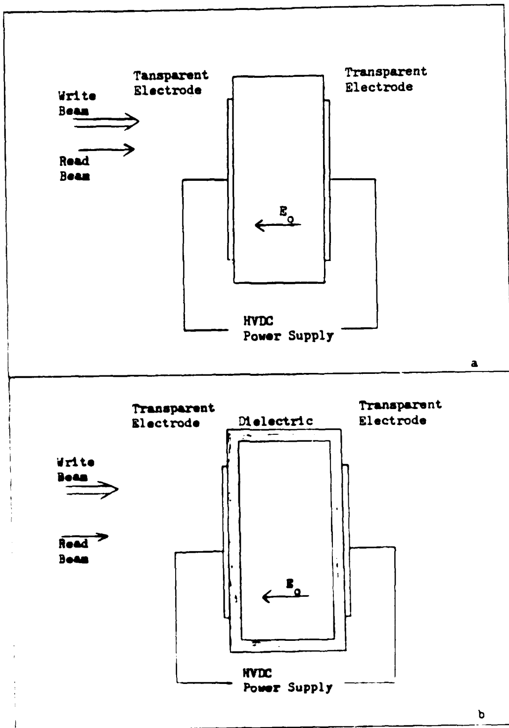
Figure 1. (a) Inducting and, (b) Standard ERL
