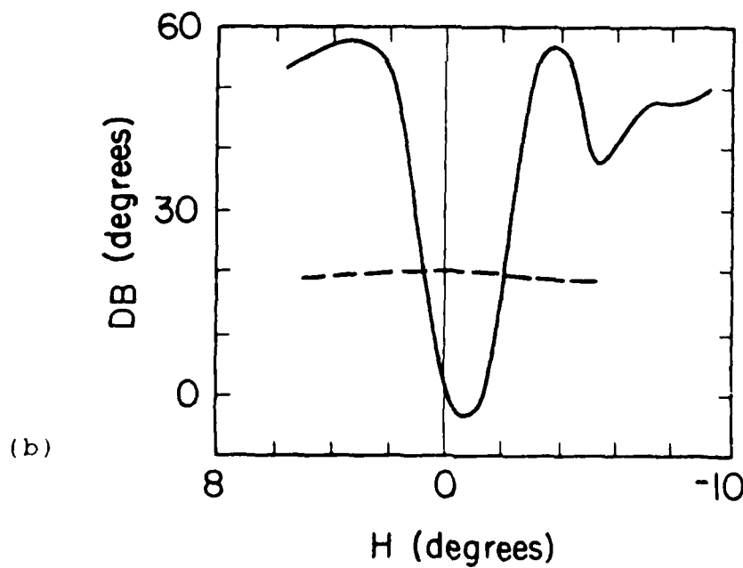
Figure 16. Values for (a) DA and (b) DB During the Very High Volcanic Turbidity Conditions at Mauna Loa, Hawaii (Adapted from Figures 14 and 15 of Coulson 11 ). The Dashed Lines are Background Values
