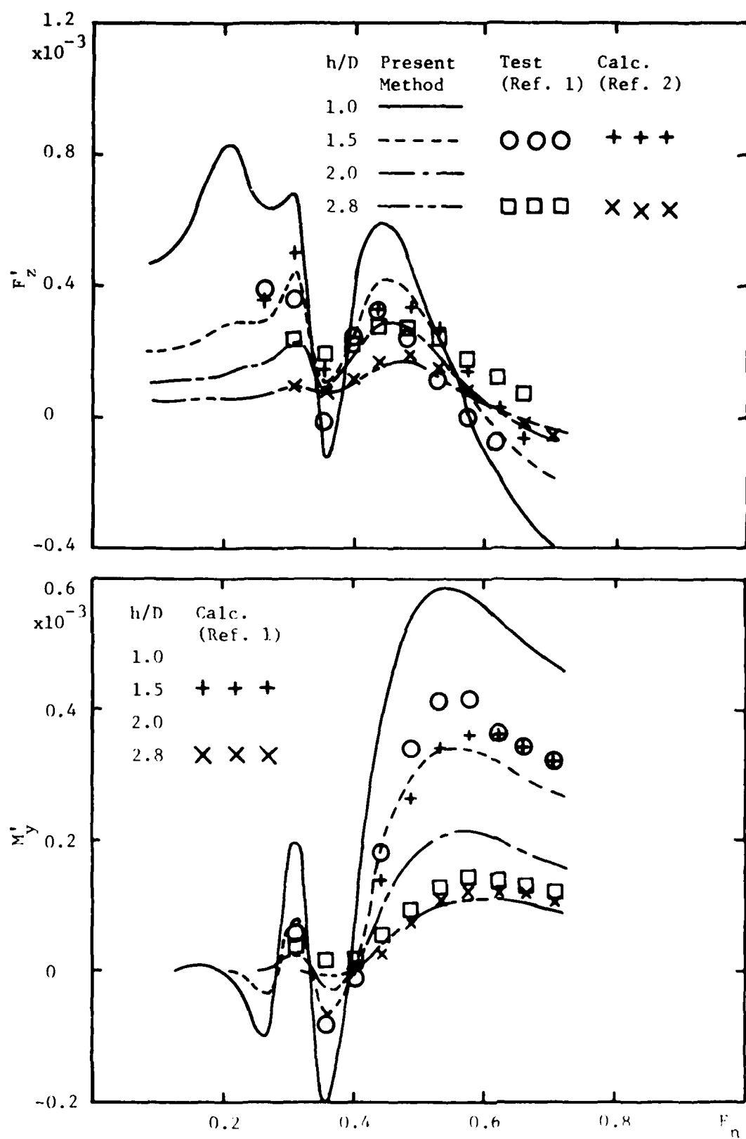
Figure 9 - Force and Moment on a Rankine Ovoid with L/D = 10.5 at Different Submergences
