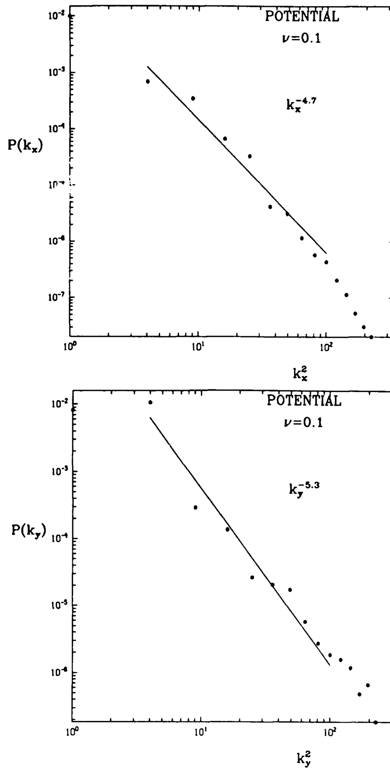
Fig. 11 — Plot of the time and transverse averaged power spectra (a) P(k_x) and (b) P(k_y) for \delta\phi for \nu = 0.10 . The units are described in Fig. 9.
