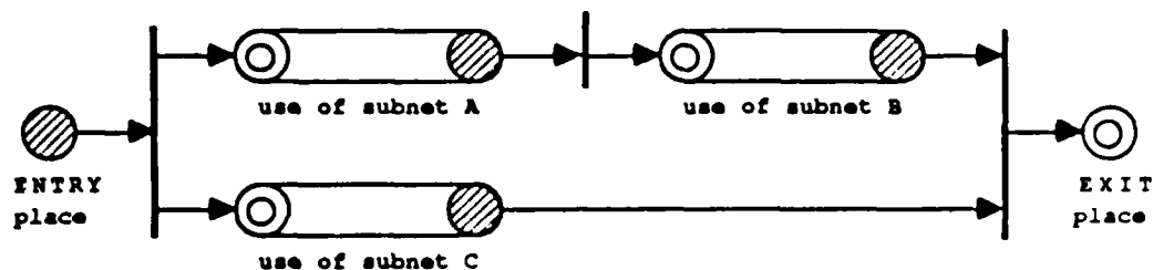
Figure 4.2: Symbolology of Subnets
