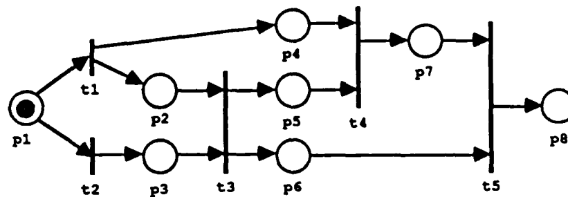
Figure 2.3: Graph of Petri Net
