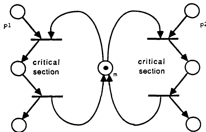
Figure 2.10: Mutual Exclusion
