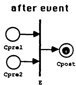
Figure 2.5: Conjunctive Transition
