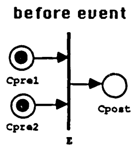
Figure 2.5: Conjunctive Transition
