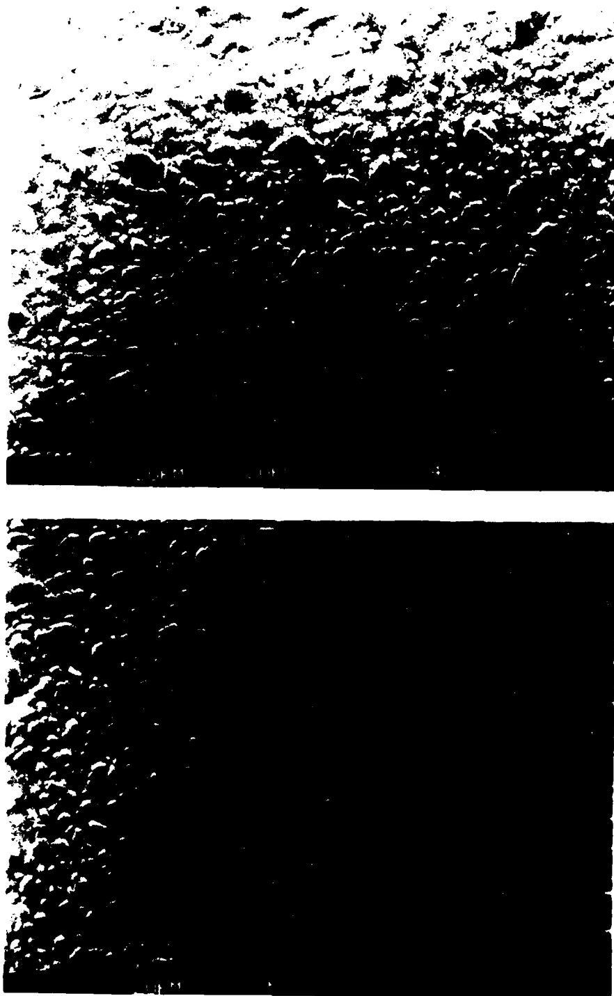
FIGURE 34 - Low Magnification SEM Micrograph Showing the SiC Distribution in the 5-30 Composite.
