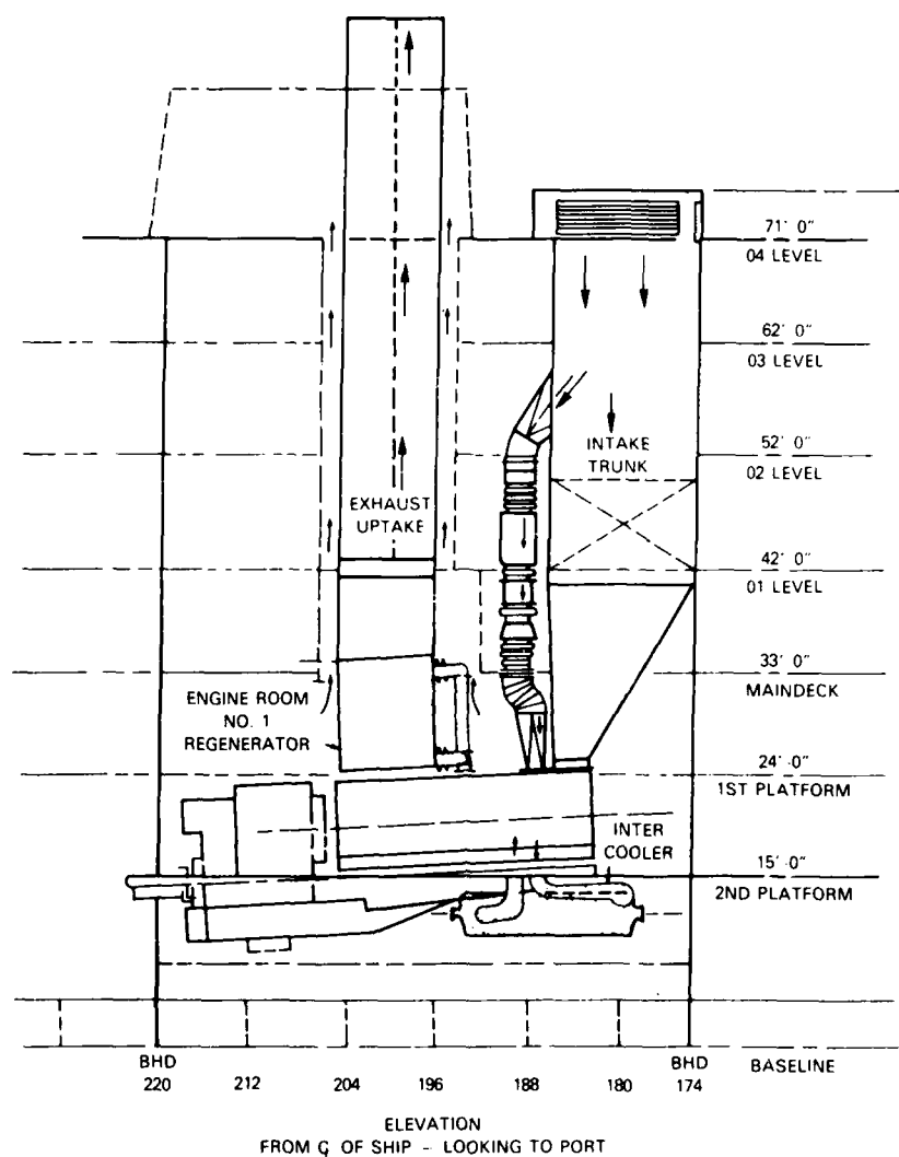
Fig. 41. Propulsion machinery.
