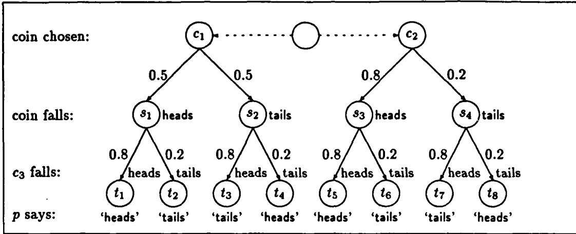
Figure 2: The system for game G_2 .
