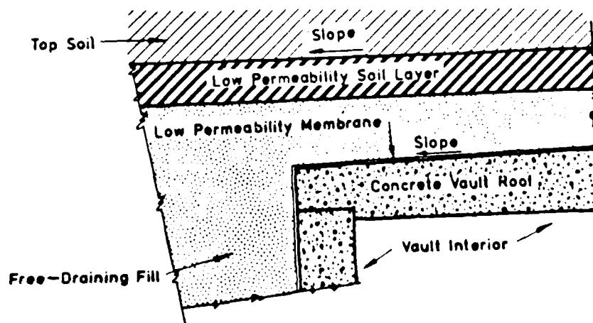
(b) Drainage blanket above and surrounding BGV
