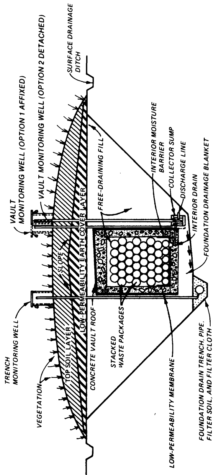
Figure 1.1. Major components of a BGV
