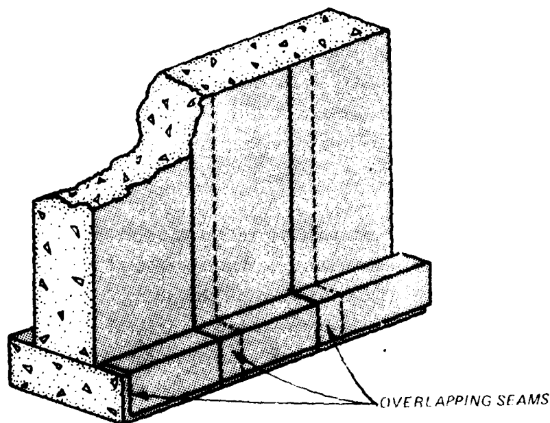
Figure 2.3.2 Low-permeability membranes applied with overlapping seams
