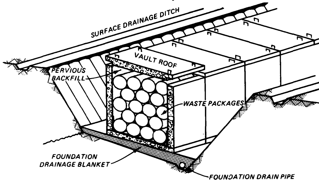
(d) Removable roof segments placed on walls (As an alternative, roof could be cast in place over free draining fill)
