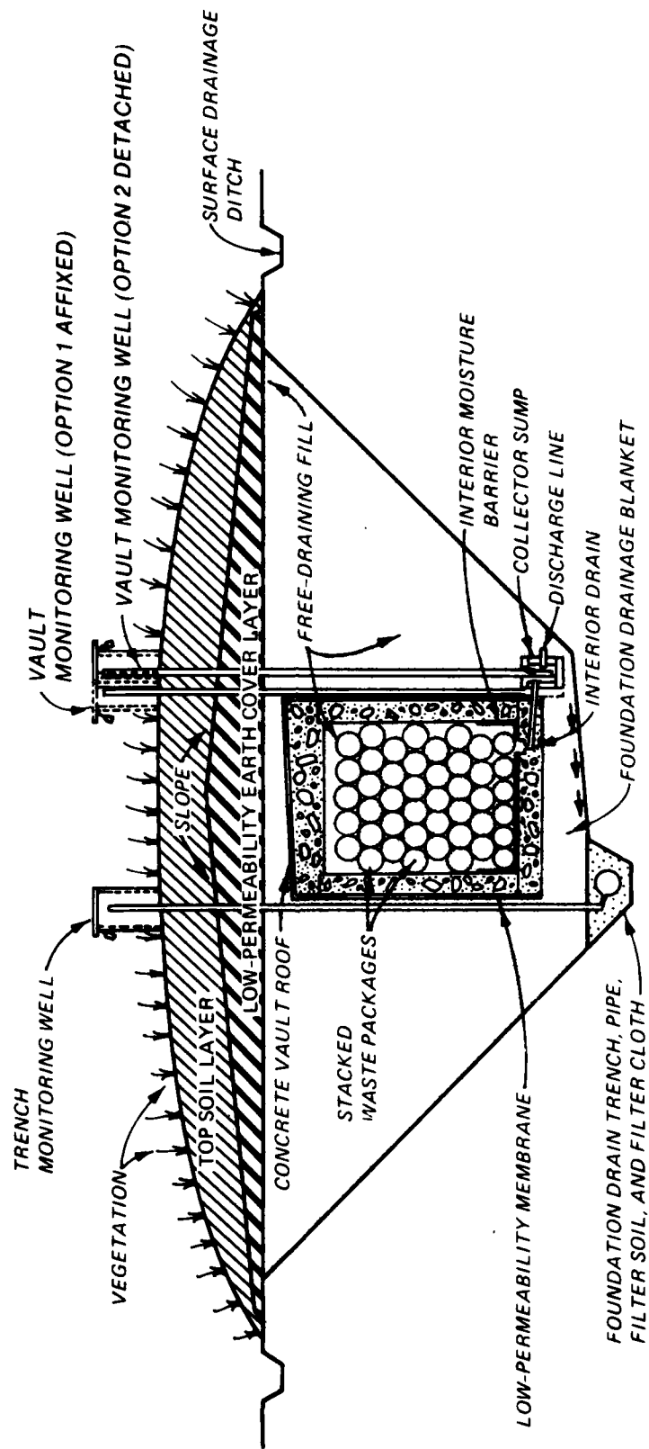
Figure 2.8.1. Major components of BGV waste cover system
