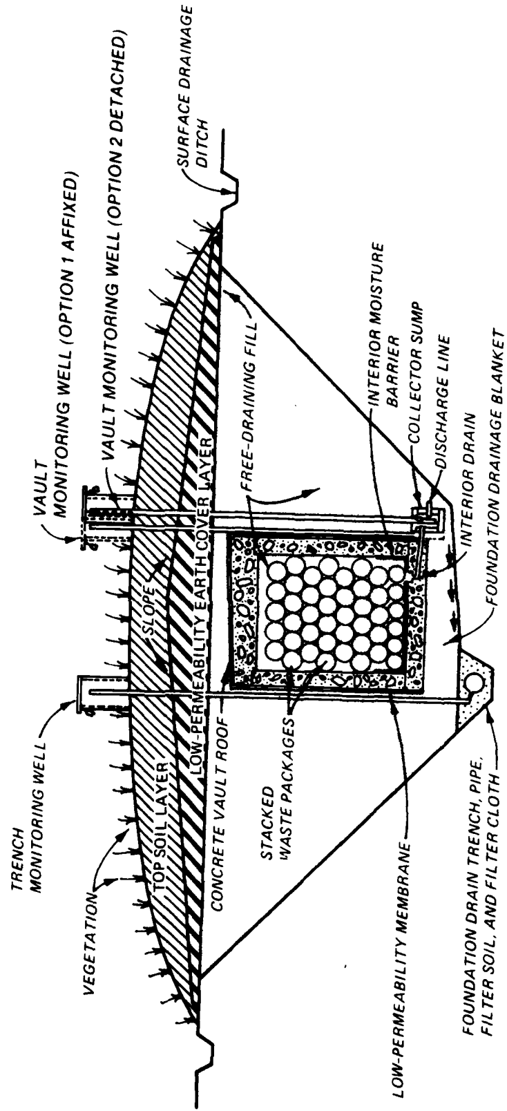
Figure 2.7.1. BGV filter and drainage system
