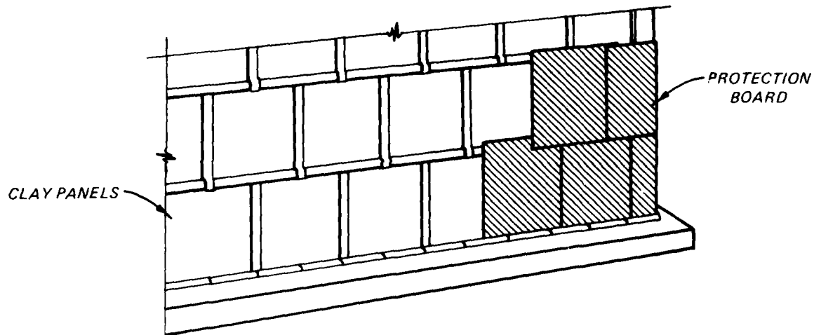
Figure 2.3.3. Bentonite panels applied to concrete
