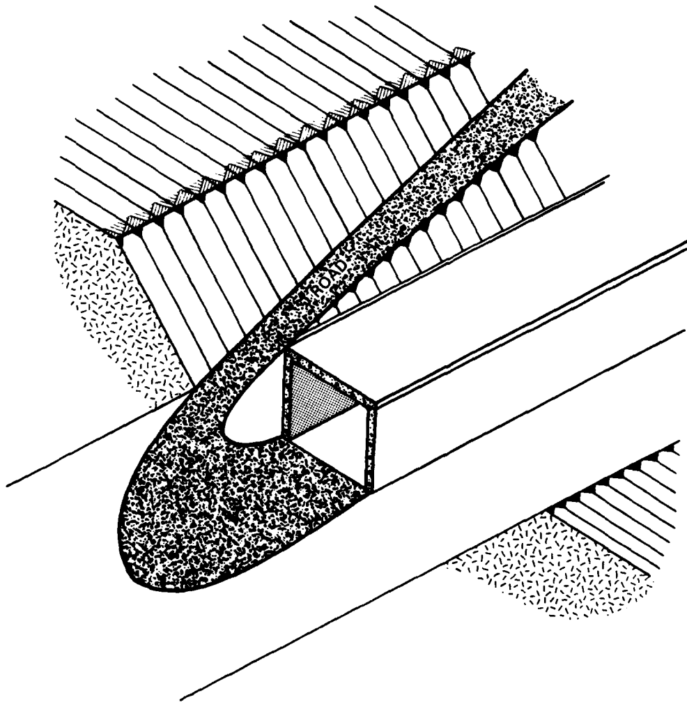
Figure 2.4.3. Side loading concept of waste emplacement in a BGV
