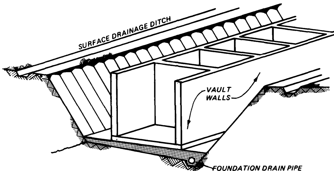
(c) Walls and divider compartments constructed
