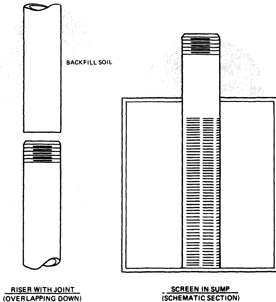
Figure 2.6.2. Features of sump monitoring wells
