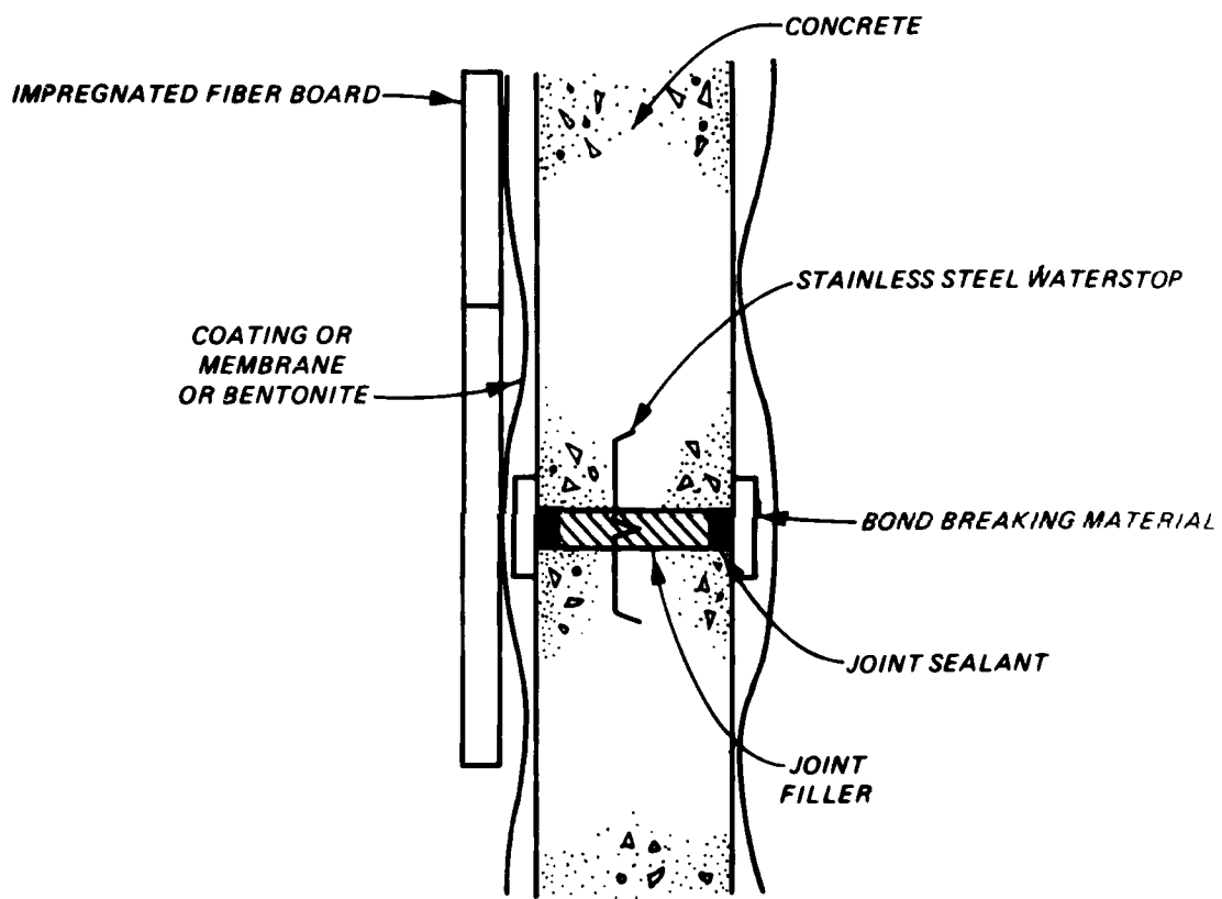
Figure 2.3.1. Locations of moisture barriers
