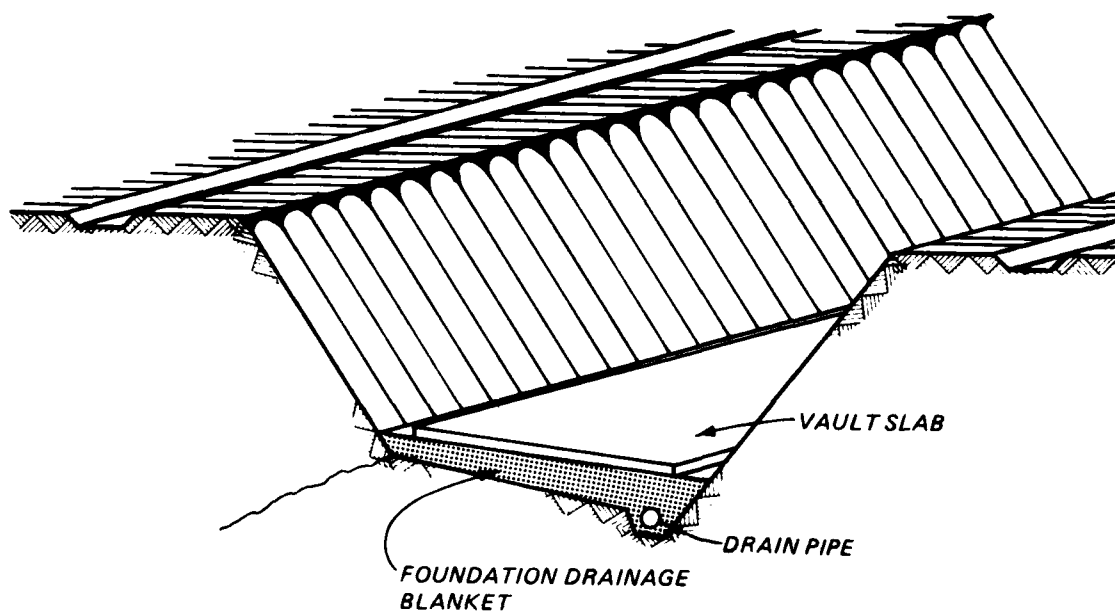
(b) Drain and floor slab
