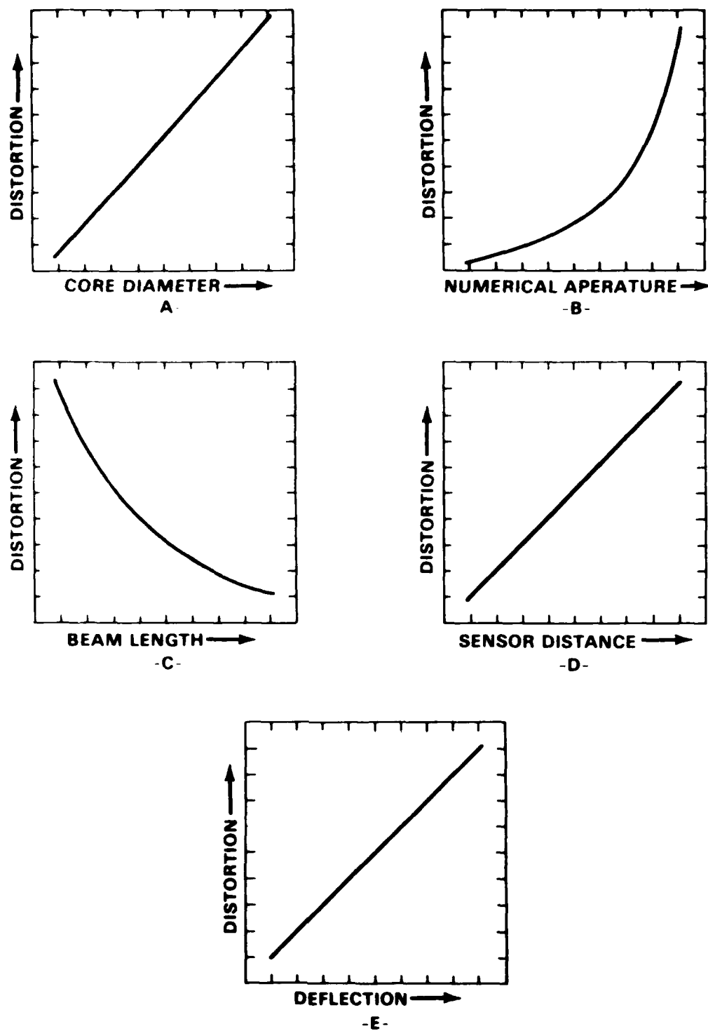
Fig. 7. Graphical representation of the trends of image distortion as a function of core diameter, numerical aperture, beam length, sensor distance, and deflection computed using equation 4.
