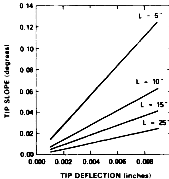
Fig. 6. Graph of the relationship between the tip slope and tip deflection for a mid-span loaded cantilever beam of different lengths, L , computed from equation 5.
