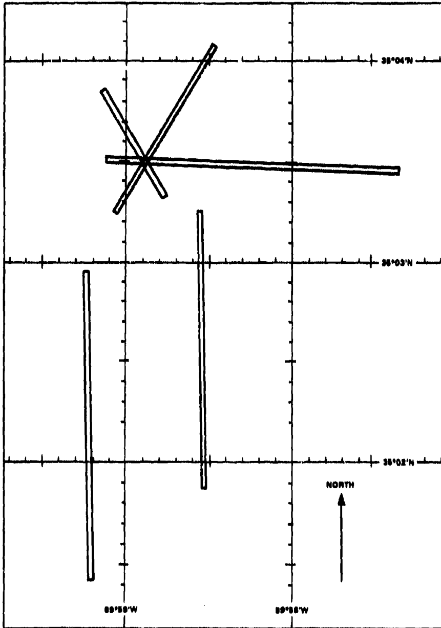
Figure IV-4: Runway layout at Memphis International Airport.
