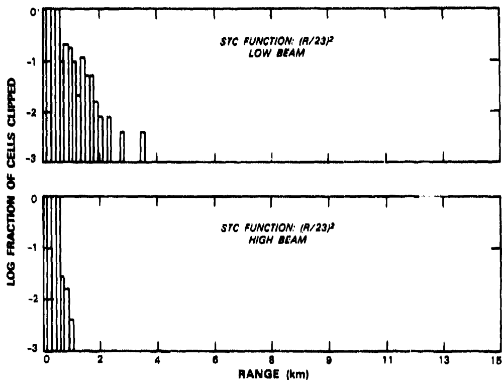
Figure IV-6a. Probability of receiver clipping (ensemble over azimuth) versus range for the ASR-8 at Memphis. As discussed in the text, an (R/23\text{km})^2 STC function is assumed.
