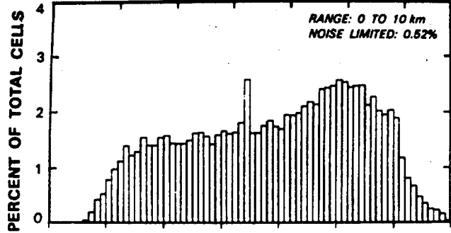
ASR-8: MEMPHIS LOW BEAM CLUTTER CROSS SECTION DENSITY (dB//1 m 2 /m 2 )
