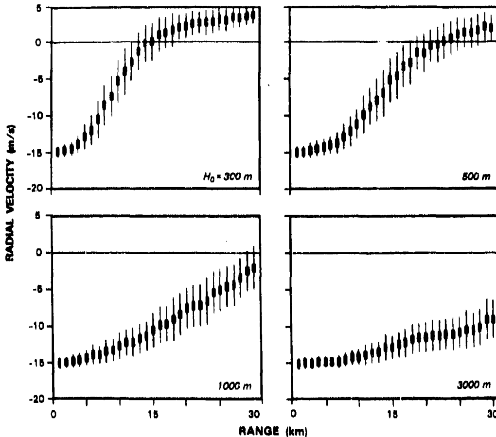
Figure III-14. Monte Carlo simulation of mean and standard deviation of pulse-pair velocity estimates versus range. The assumptions are as in Figure III-2, except that use of the synthesized maximum signal to precipitation interference channel is assumed as in Figure III-10(a).
