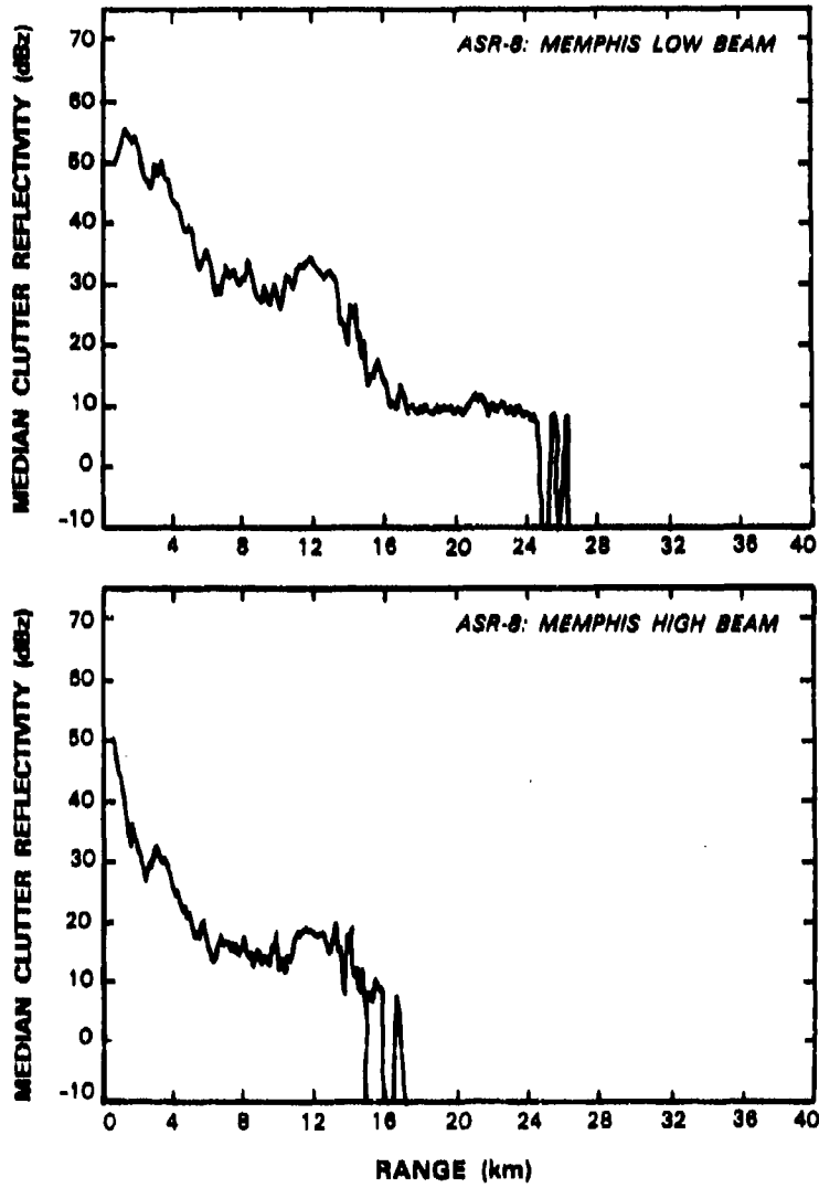
Figure IV-3a. Median ground clutter intensity (ensambled over azimuth) versus range for the ASR-8 at Memphis International Airport.
