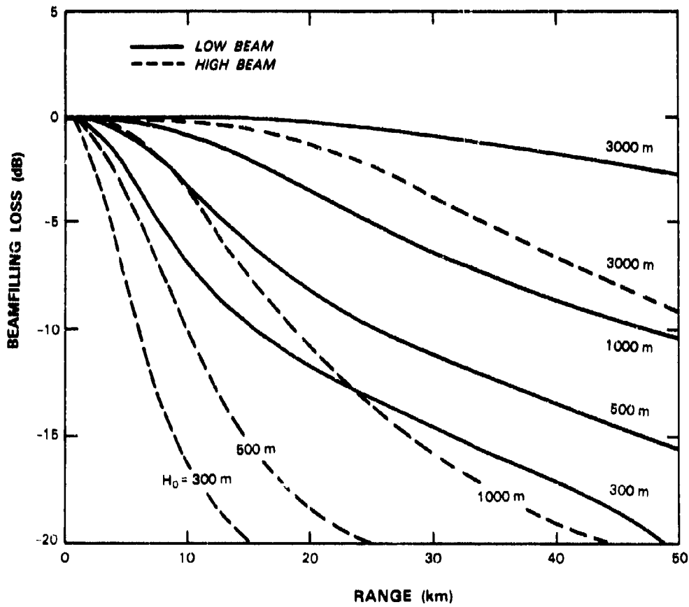
Figure II-6. Beamfilling loss versus range for an ASR-9. The different curves are for echoes extending from the surface to the indicated heights.
