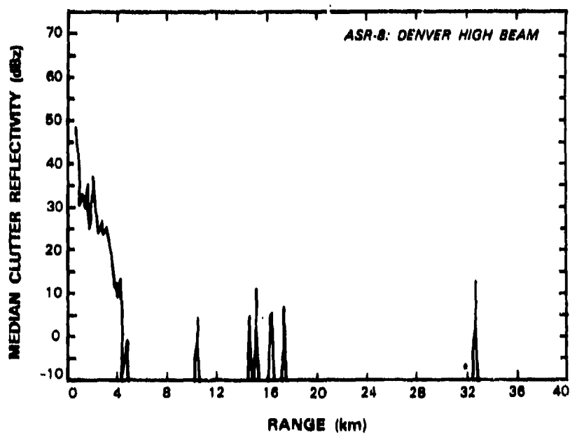
Figure IV-8b. Median ground clutter intensity (ensembled over azimuth) versus range for the ASR-8 at Stapleton Airport.
