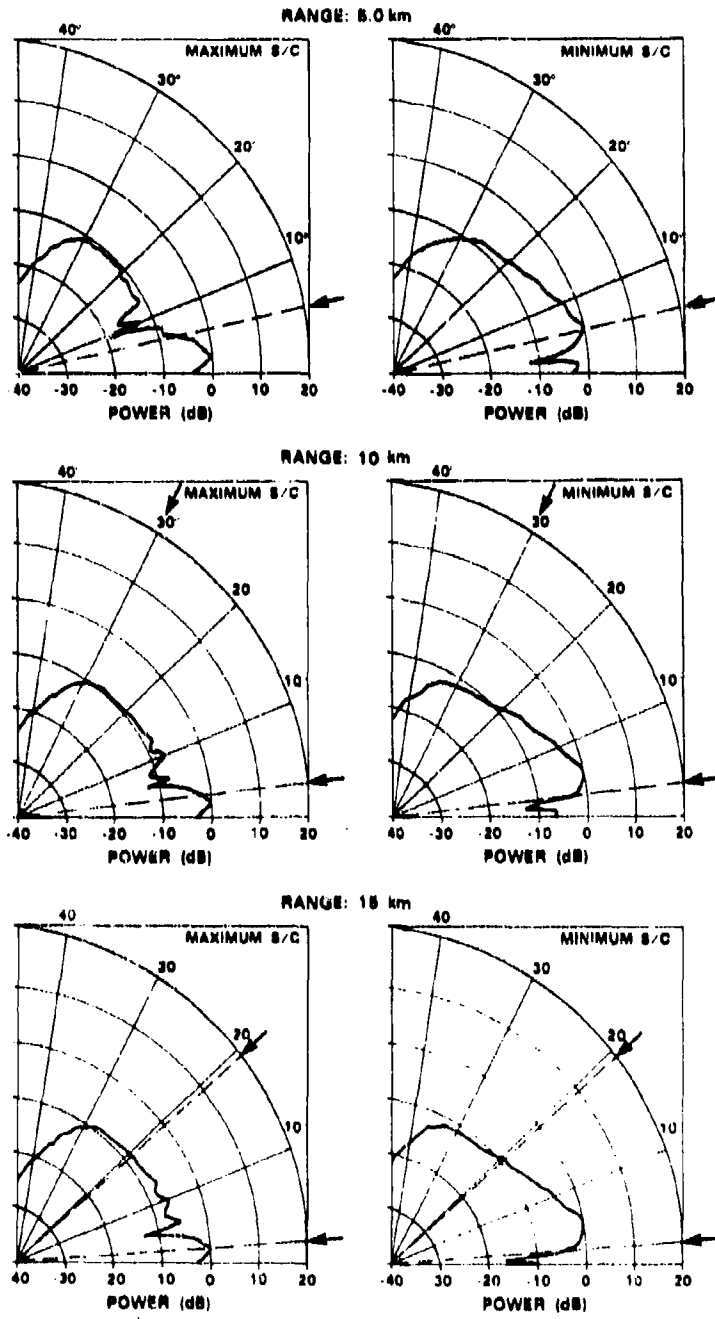
Figure III-12. Effective one-way power beam patterns for signals synthesised through coherent combination of high and low beam signals as described in the text.
