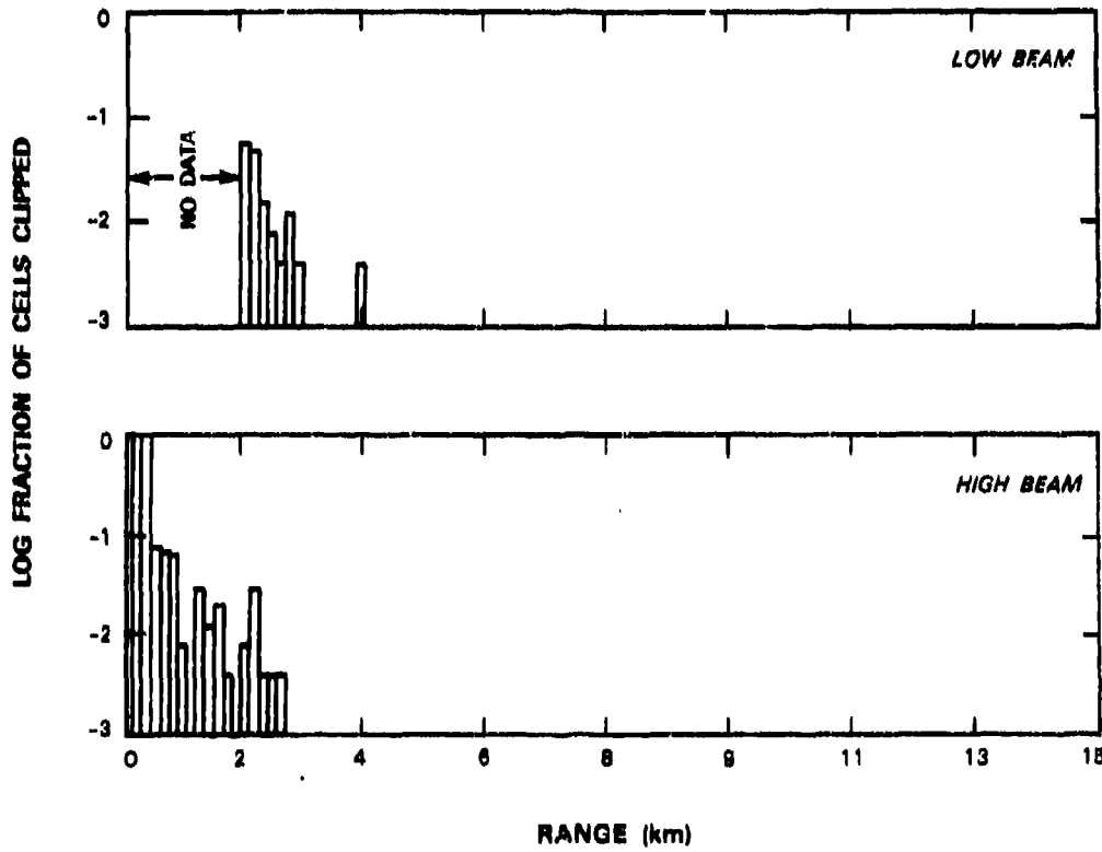
Figure IV-6b. Probability of receiver clipping versus range for the ASR-8 at Denver, assuming an (R/23km)^3 STC function.
