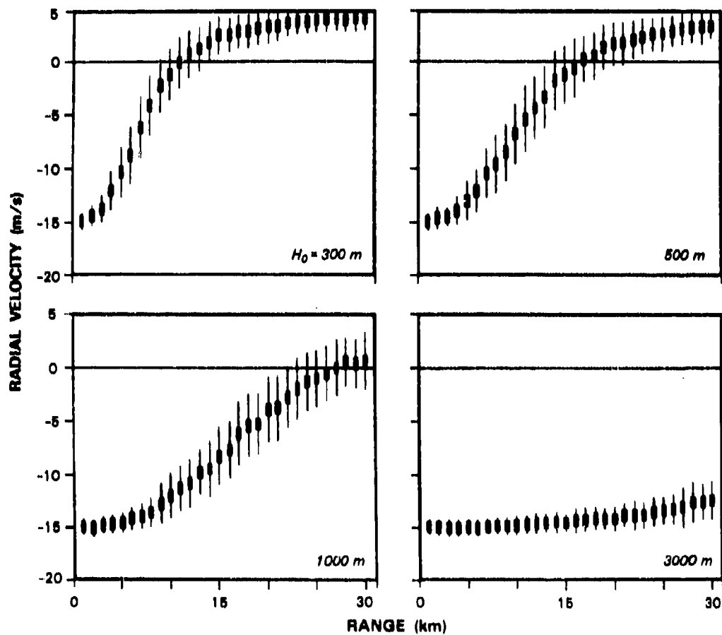
Figure III-2. Monte Carlo simulation of mean and standard deviation of pulse-pair velocity estimates versus range. Each plot assumes: (i) uniform reflectivity from the surface to 10 km; (ii) an outflow layer from the surface to the indicated height where the radial velocity component is -15\text{ ms}^{-1} ; (iii) radial velocity of 5\text{ ms}^{-1} at all altitudes above this layer. The simulation assumed that the low receiving beam is used.
