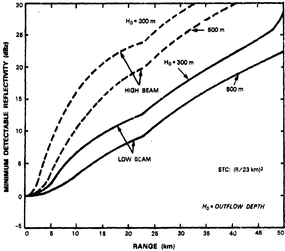
Figure II-7. ASR-9 minimum detectable weather reflectivity factor including the beamfilling losses for a 300 or 500 m deep thunderstorm outflow layer. An (R/23\text{ km})^2 STC function is assumed.
