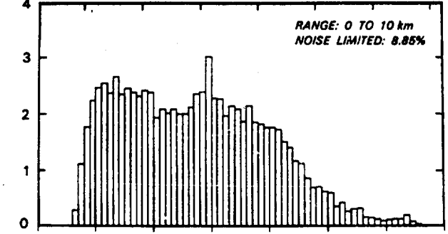
ASR-8: MEMPHIS HIGH BEAM CLUTTER CROSS SECTION DENSITY (dB//1 m 2 /m 2 )
