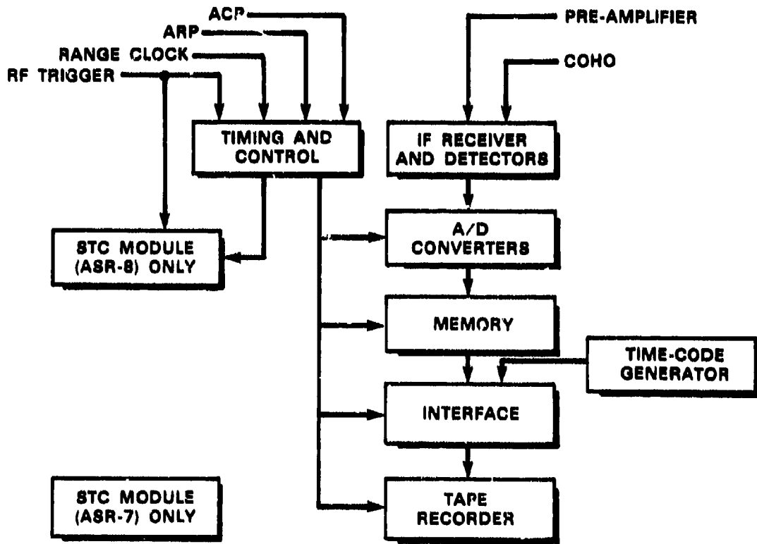
Figure C-1. ASR ground clutter recording system.
