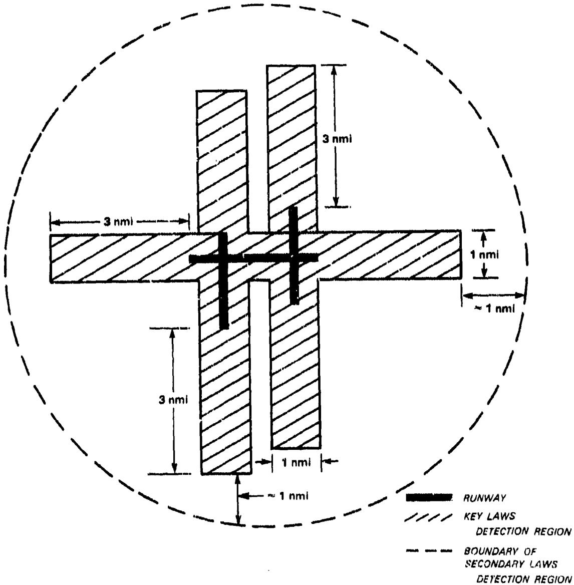
Figure 1-3. Principal microburst detection area for a hypothetical airport.
