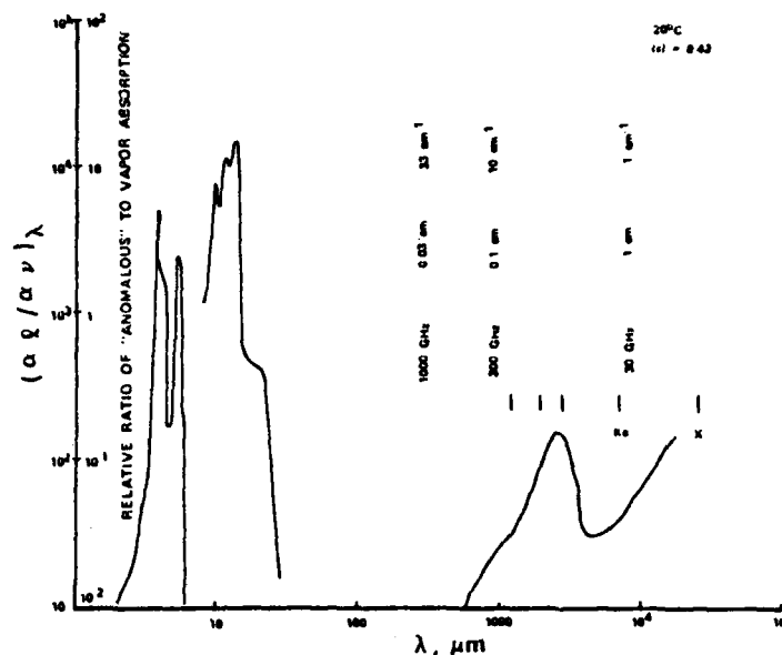
Figure 32. Ratio of Molecular Absorption Coefficients for Liquid Water and Water Vapor, vs. Wavelength.
