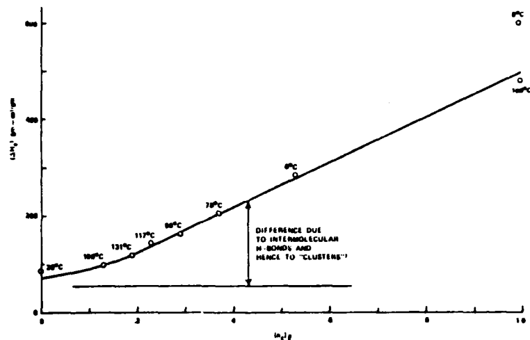
Figure 14. Latent Heat of Vaporization, \Delta H_v , vs. Weight Fraction of "O-H" in Molecule; Pure Liquid Water Corresponds to (n_c)_L = 1.0 .
