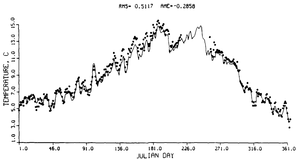
Figure 5. Predicted (—) and observed (...) stream temperature data for 1978 (Sheet 1 of 3)
