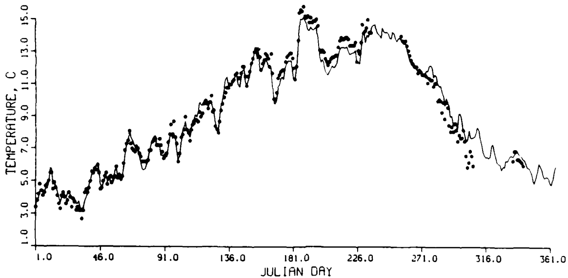
Figure 4. Predicted (—) and observed (...) stream temperature data for 1979 (Sheet 1 of 3)
