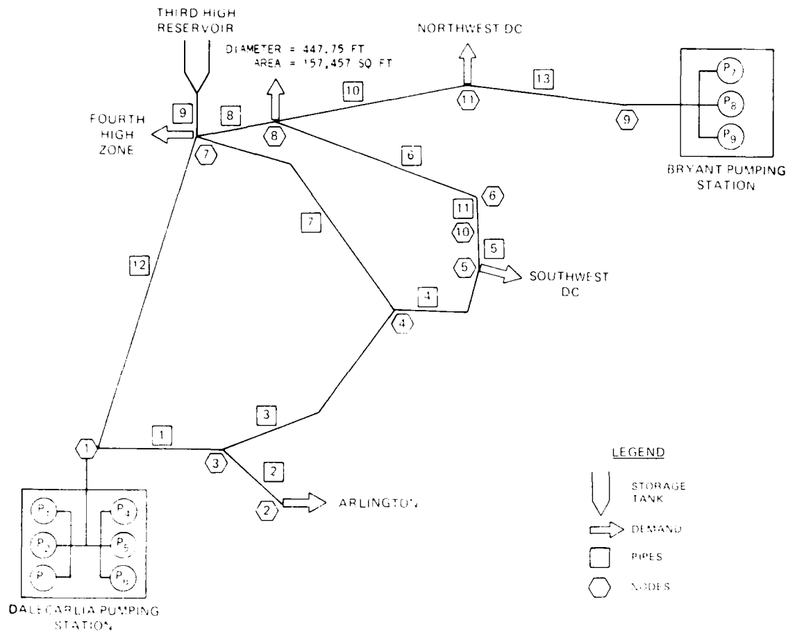
Figure 12. Schematic of third high-pressure zone
