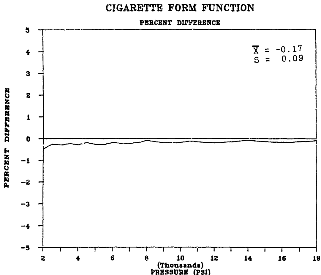
Figure 2. Percent difference between computed burn rates from MINICB and theoretical burning rates for a cord burning in a cigarette fashion. Validation 1.
