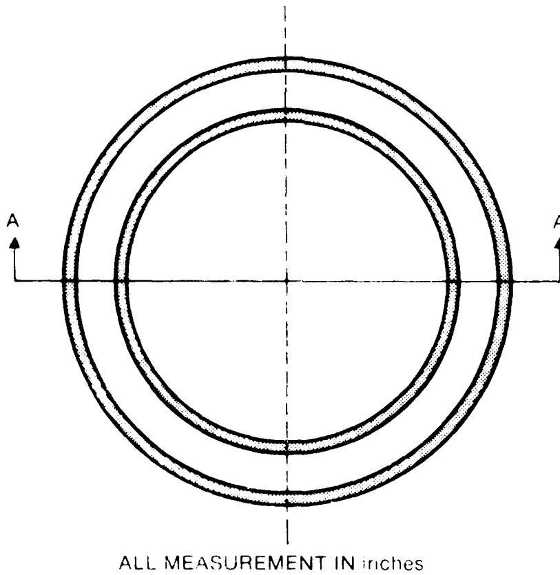
Figure 27. Dimensions of the end cap for the Model 1 ceramic chamber.
