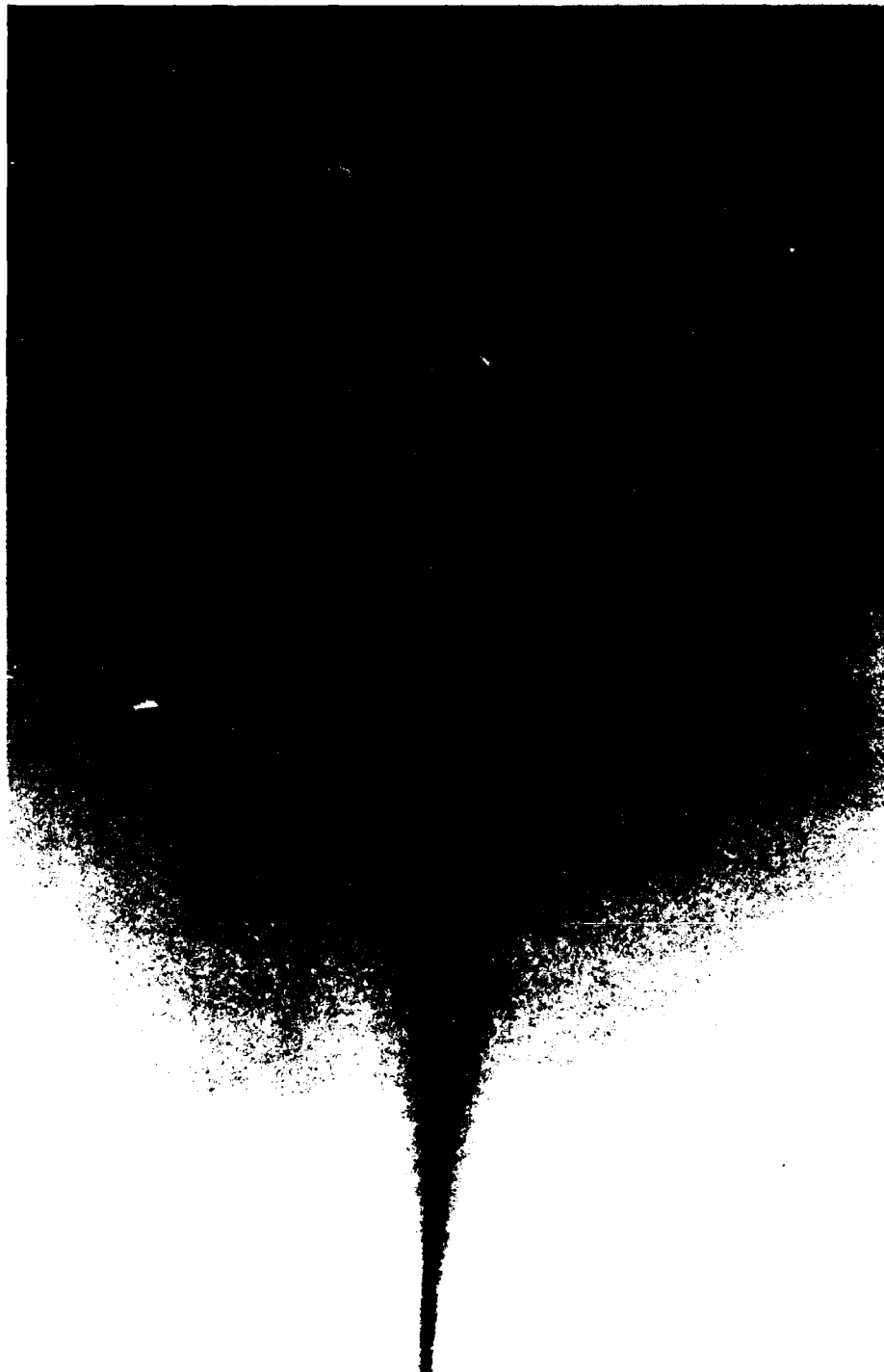
Figure 19. Closeup of the brazed joints between the individual ceramic rings.
