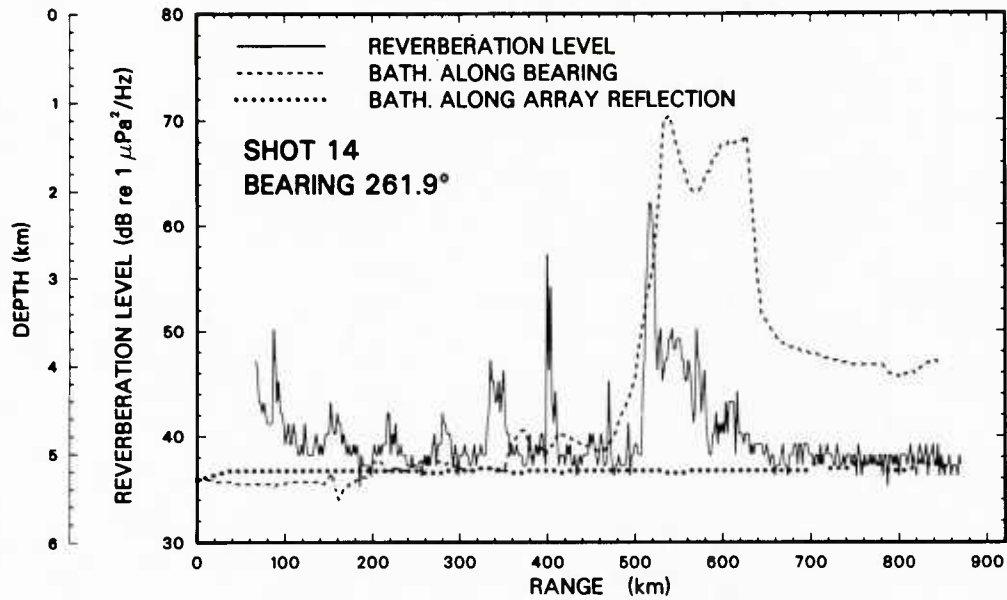
Fig. 20 — Sample plot from program REVBMSCAT. This plot shows reverberation power spectral density (dB re 1 \mu\text{Pa}^2/\text{Hz} ) vs range along primary radial of Fig. 19 from our digital map file MP12.DB. Slight differences between this curve and that of Fig. 19 are due to the fact that this great circle radial may span more than one beam as it goes out in range; and our reverberation levels are converted to integer byte format for compatibility with our COMTAL image monitor. Near range bottom reverberation (inside of about 65 km) is omitted from our single-shot map files, hence the short gap at left. Also superimposed to same range scale is SYNAPS bathymetry for primary radial (dashed) and conjugate radial (dotted).
