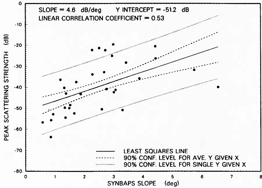
Fig. 4 — Peak scattering strength measure vs SYNAPS bathymetry slope
