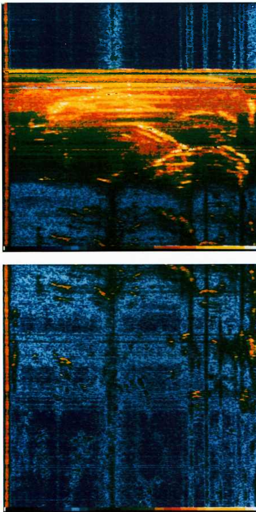
Fig. 14 — Example of data in a beamtime format. This is received power spectral density (color coded); black—lowest, white—highest; each subplot is for about 2 minutes of data; there is slight overlap between the two subplots (see text for description).
