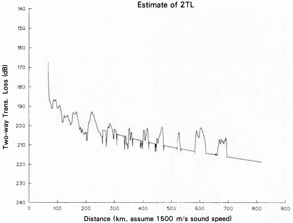
Fig. 24 — Sample plot from program GETTL. Two-way transmission loss vs range estimate for shot 12; used for creating a single-shot scattering strength beam-time file SS12.DB with program SS (see text and Appendix B).
