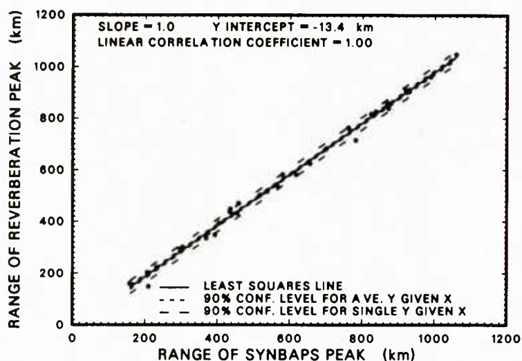
Fig. 6 — Range of reverberation peak vs range of SYNBAPS bathymetry
