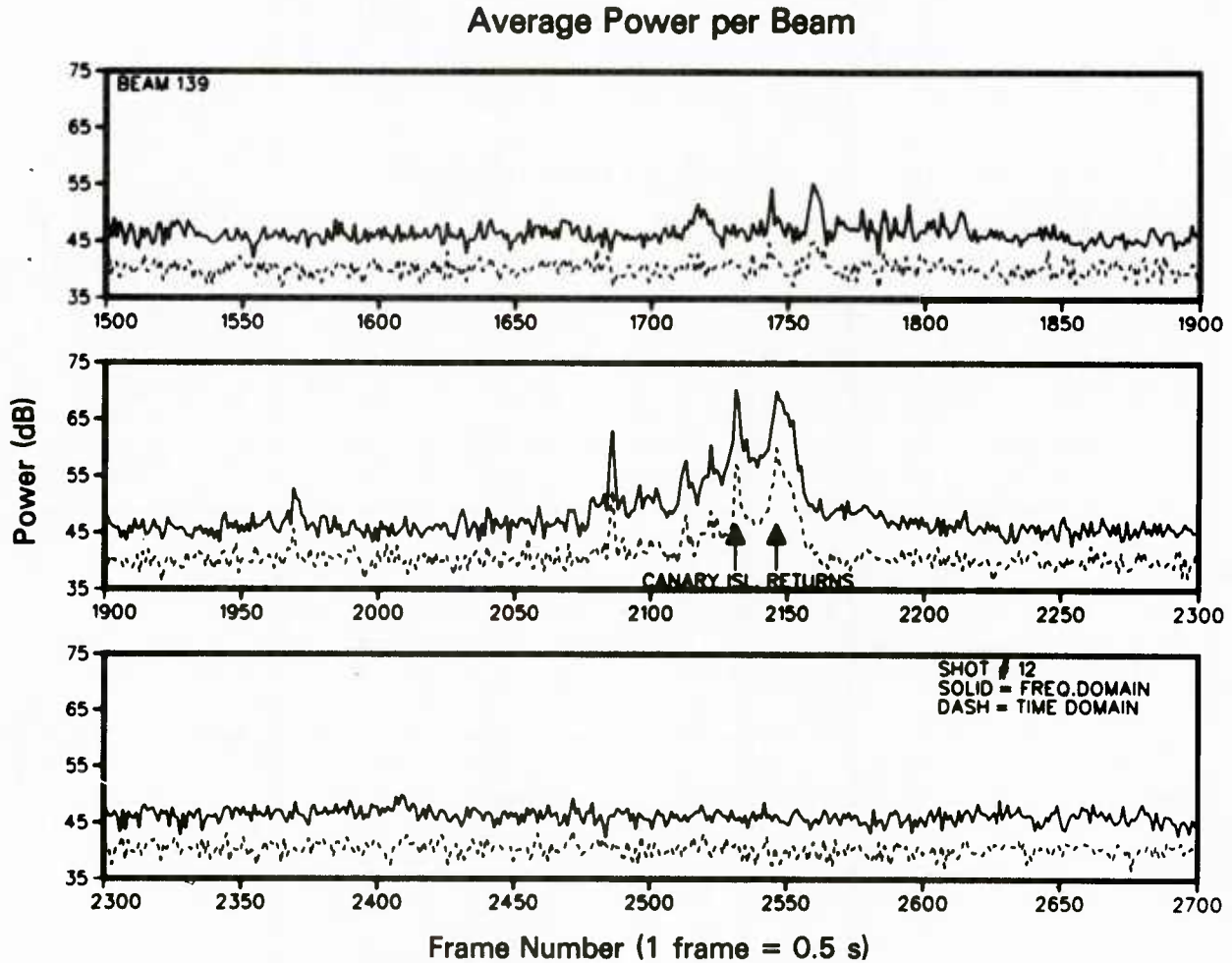
Fig. 10 — Continuation of Fig. 9 but only one beam (No. 139; pointed toward Canary Islands)
