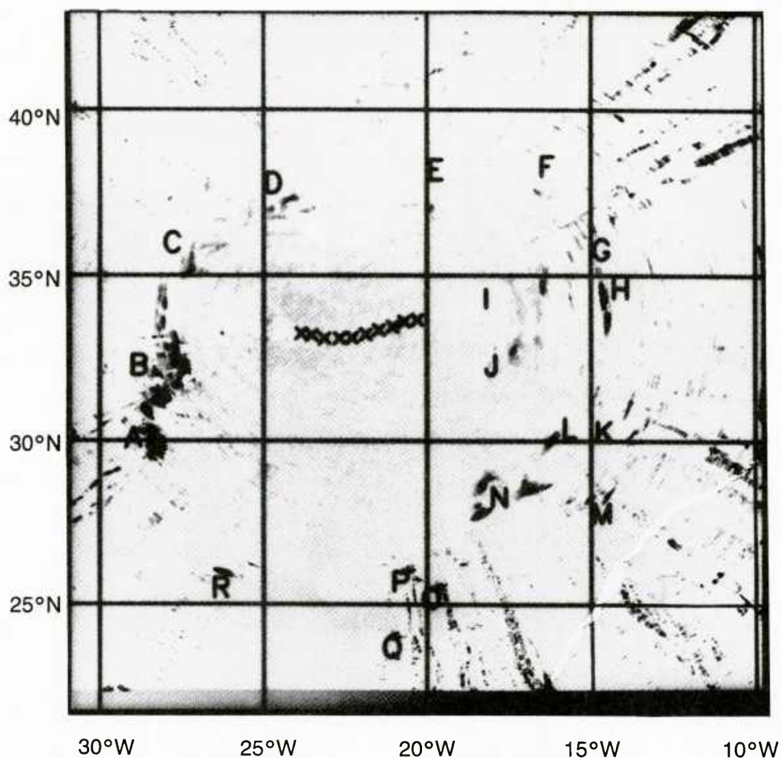
Fig. 8 — Integrated reverberation-bathymetry map for Canary Basin. Created by averaging single-shot maps for shots 10 through 19 as described in text. Map is 21^{\circ} 20' on each side (about 2371 km north-south \times 1988 km east-west). Each map pixel is about 1.0 in size. Range of grayscale is from 6400 m (darkest) to 0 m (lightest).
