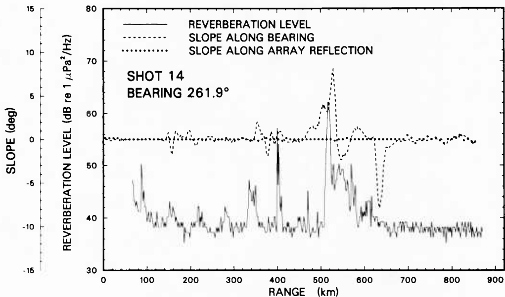
Fig. 21 — Sample plot from program REVBMSCAT. Similar to Fig. 20, but with SYNAPS bathymetric slopes instead of depths.
