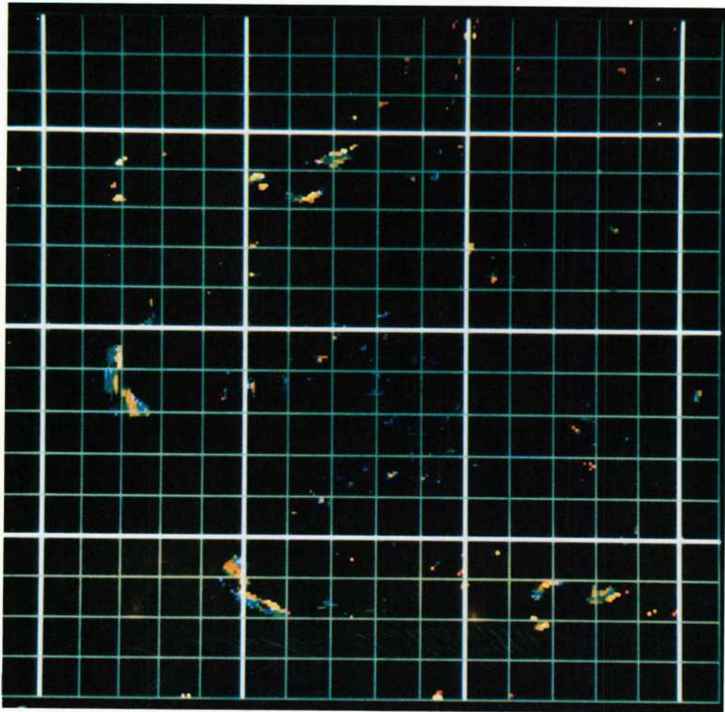
Fig. 26 — Example of single-shot scattering strength map (shot No. 12). Scattering strength is color coded; lighter colors indicate higher scattering strength. Each topographic backscatter feature appears twice on this map because of the left-right ambiguity of the linear receiver array (see text).
