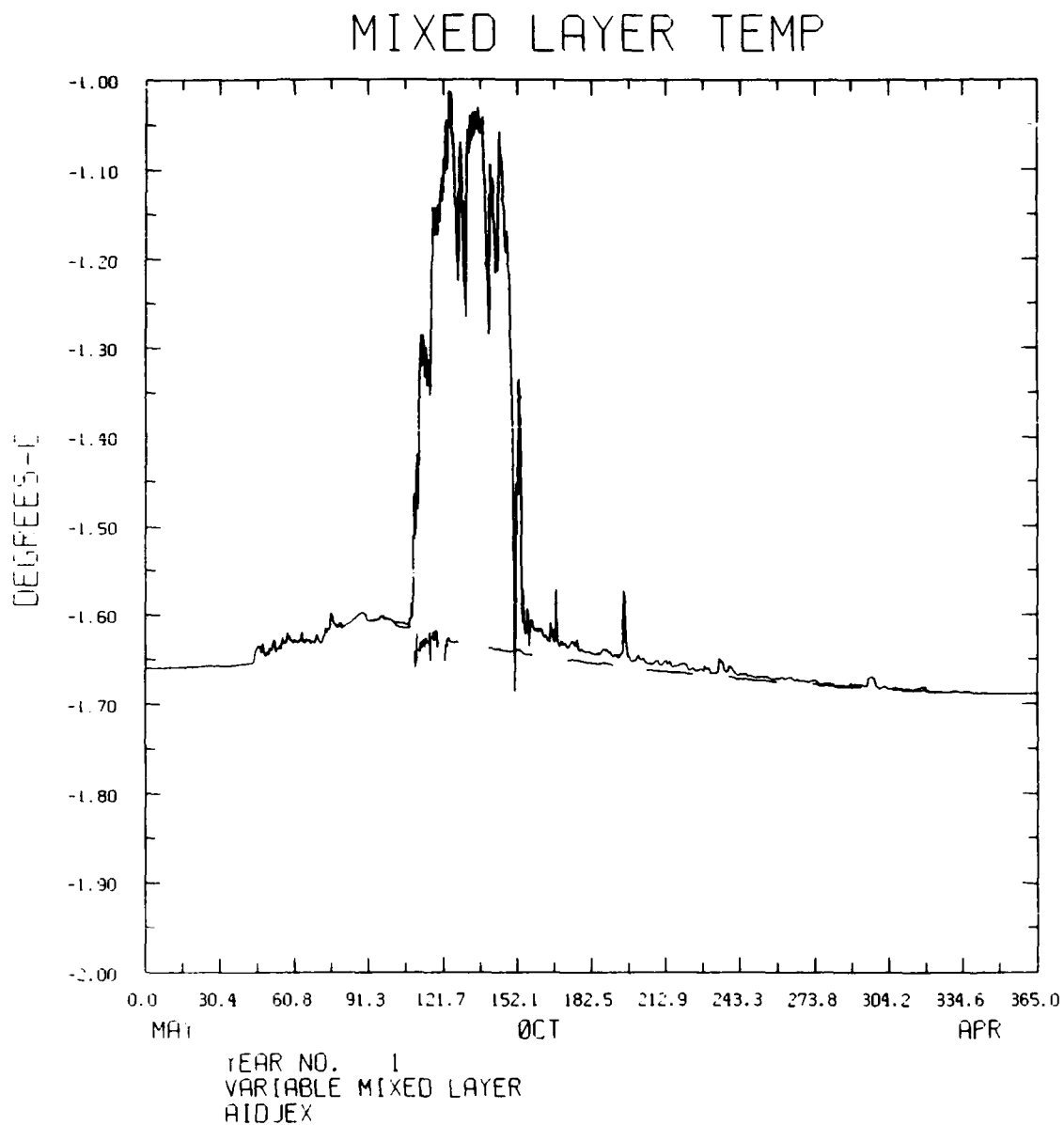
Figure 79. Comparison of mixed-layer temperature for Case 3N and Case 3O. Open water occurred in both cases. Case 3N is the dashed curve, and Case 3O is the solid curve.
