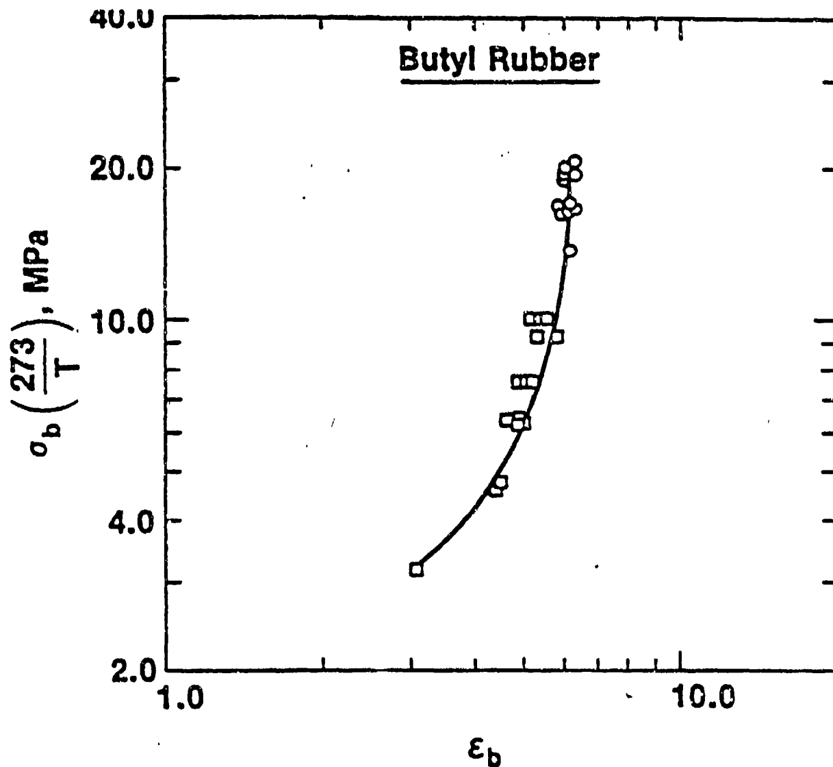
Figure 3.3 Typical failure envelope for a carbon black filled butyl rubber. (o) From constant rate of deformation measurements. ( \square ) From creep to failure measurements. [After McKenna and Zapas(2).]
