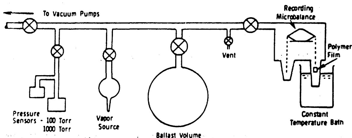
Figure 2. Vapor sorption apparatus.
