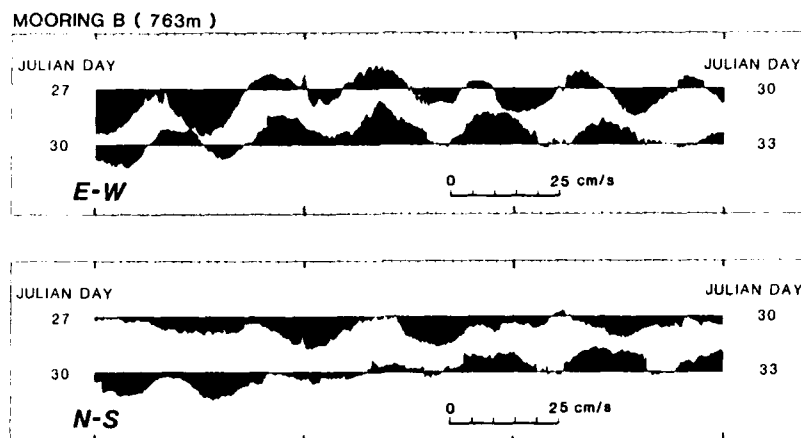
Fig. 56. Train of internal nonlinear waves (solitons) in southern Alboran Sea. [Position B and depth of 763 m. Signal of nonlinear waves is superimposed on tidal variation. E-W, N-S signify the velocity components with the eastward and northward direction positive-up.]
