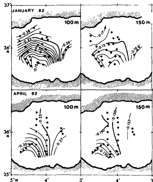
Fig. 32. Contours of dynamic height anomaly in dynamic meters for the depths of 100 and 150 m (relative to 200 m) from January and April 1982. [They show broad anticyclonic circulation. Dots signify the positions of CDT casts.]
