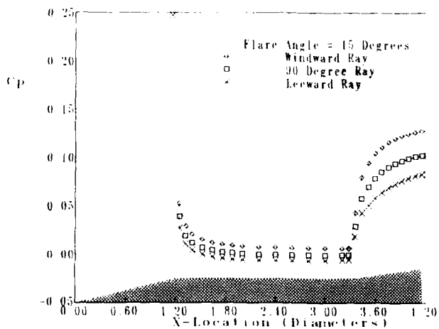
Figure 12. Pressure coefficient distribution for cone-cylinder-flare for 15° flare.
