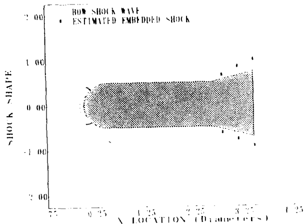
Figure 2. Shock shape of hemisphere-cylinder-flare for 15° flare.
