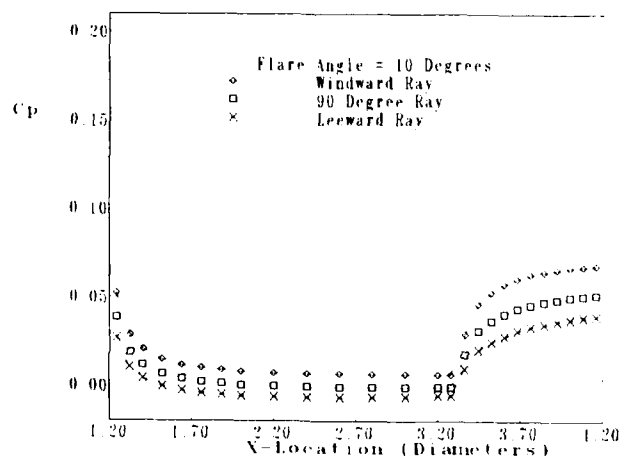
Figure 15. Pressure coefficients distribution for cone-cylinder-flare for 10° flare.
