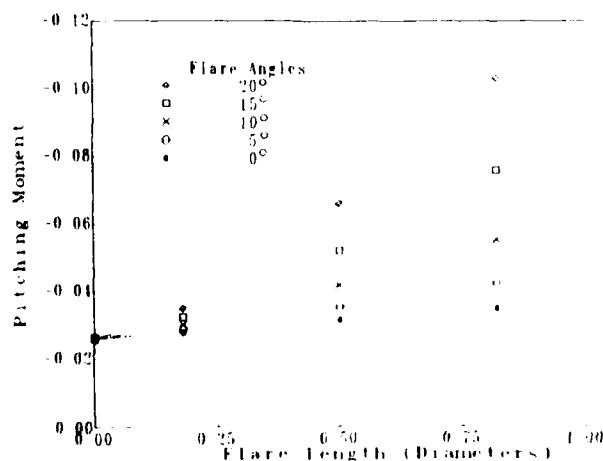
Figure 16. Pitching moment curves for cone-cylinder-flare for 0, 5, 10, 15, and 20 degree flares.
