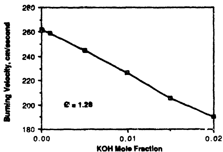
Figure 6. Burning Velocity vs [KOH]
